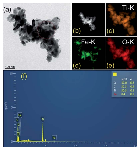
Fig. 4 (a) The TEM image, (b) HAADF-STEM image, (c) Ti, (d) Fe and (e) O elements mapping images and (f) EDS spectrum of TF0.5.
