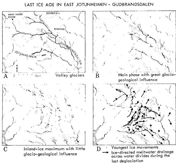
Fig. 7. A reconstruction of 4 phases of ice movements during the last ice age (after Garnes 1975).
