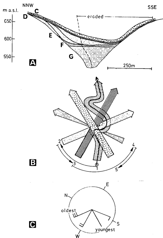
Fig. 15. Genetic interpretation of the basal tills at Stenseng.
