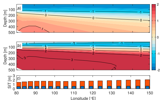
FIG. 13. (a),(b) Ensemble mean winter temperature ( ^{\circ}\text{C} ) during the recent decade (2010–19) and in the future (2070–79) in a section crossing the eastern Arctic Ocean (see location in Fig. 12). (c) Winter sea ice thickness (SIT) along the section for the two periods (2010–19: red; 2070–79: blue).
