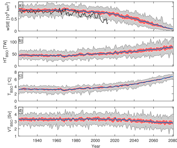
FIG. 2. Time series of (a) winter sea ice extent (wSIE) in the Barents Sea, (b) heat transport through the BSO ( HT_{BSO} ), (c) average temperature ( T_{BSO} ), and (d) volume transport of the BSO inflow ( VT_{BSO} ). Blue line: ensemble mean; red shading: interquartile range; gray shading: ensemble spread. The black line in (a) shows the observation-based winter sea ice extent from Walsh et al. (2017).
