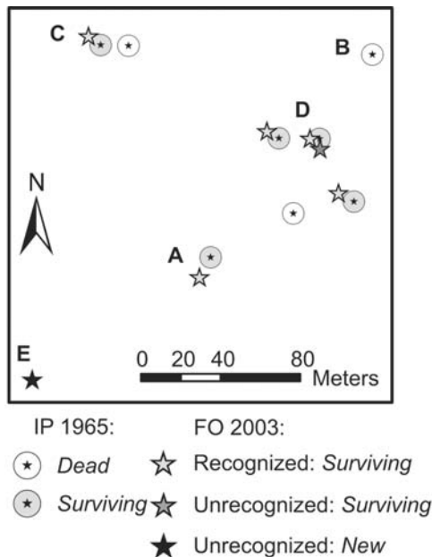
Figure 3. Change Categorization; an example from Wadi Gaetri. Distance is measured from each interpreted point (IP) to the nearest field observation (FO) with canopy area >6\text{ m}^2 . A If an IP has only one FO closer than 20 m, the two points are considered as referring to the same tree and categorized as surviving . B If an IP is separated by more than 20 m from any FO it is considered unmatched and categorized as dead . C If two IPs have the same FO closer than 20 m, the pair with the shortest distance is considered as referring to the same tree and the IP categorized as surviving . The second IP is categorized as dead if no other FO is closer than 20 m. Unmatched FOs are categorized as unrecognized and can be either D accounted for and merged with surviving or E not accounted for and merged with new (cf. [32]). doi:10.1371/journal.pone.0000208.g003
