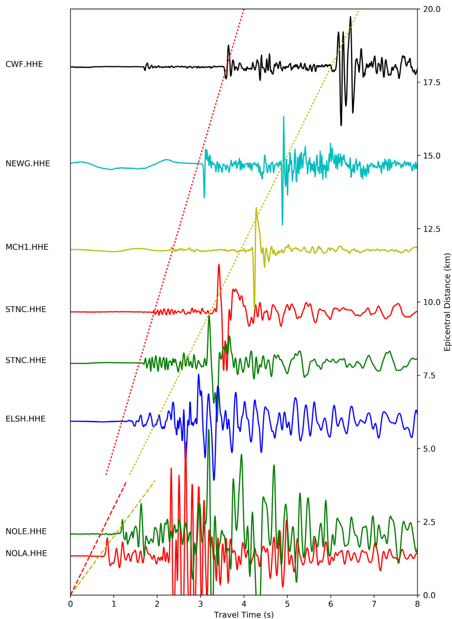
Figure 10. Waveforms at a selection of distances from various earthquakes in the UK data set. The dotted lines show typical Pg (red) and Sg (yellow) velocities of 5 and 3 \text{km s}^{-1} . The dashed lines show Pg (red) and Sg (yellow) for shallow crustal paths (3 and 2 \text{km s}^{-1} ). For the stations closer than about 10 km, Sg can be clearly seen but is much smaller than a later arrival (seen at about 2.25 s on NOLA and NOLE), which does not have a constant velocity across the traces.
