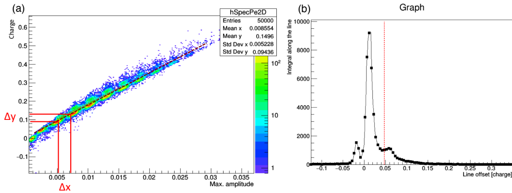
Figure 7. (a) Scatter plot of integrated charge versus maximum amplitude at waveform minimum and (b) the projection orthogonal to the dashed line. The peak represents all contributions of photoelectron peaks that are not affected by afterpulsing while the small peak to the right shows photoelectron peaks affected by afterpulsing.
