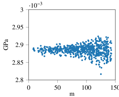
FIGURE A3 Oscillations in the normal component of the Lagrange multiplier. Left: The negative normal component of the Lagrange multiplier -\lambda on the fracture. Right: The negative normal component of the Lagrange multiplier -\lambda , where the x-axis is the radial distance from the fracture center, ie, the center is at x = 0 , whereas the tip is at x \approx 150 m [Colour figure can be viewed at wileyonlinelibrary.com]
