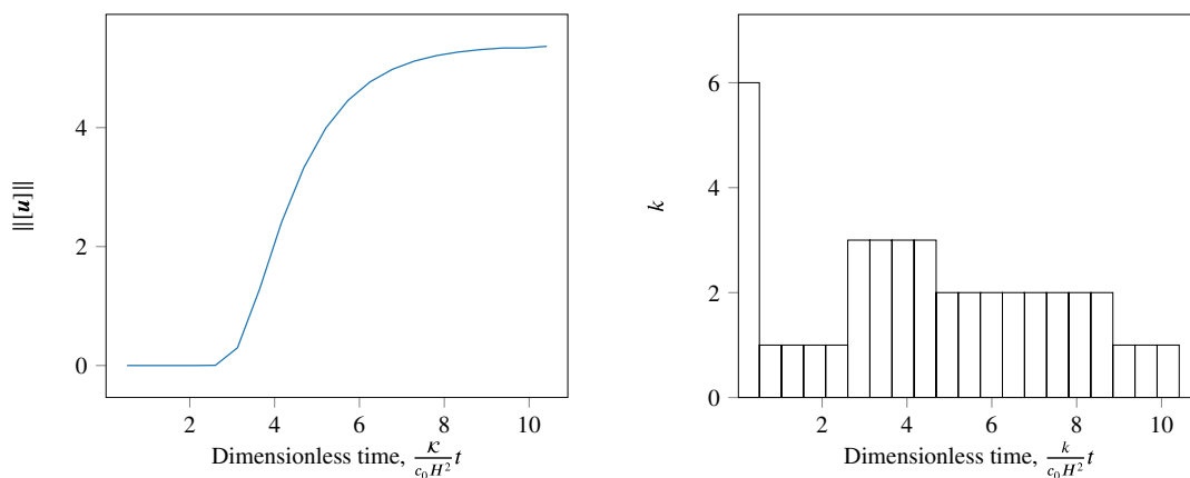
FIGURE 11 Results from Example 4. The length scale H=600 m is the height of the domain. Left: Slip distance as a function of time. Right: Convergence of the Newton solver. Each time step is represented by a rectangle, and the y-axis shows the number of Newton iterations needed until the convergence tolerance is reached [Colour figure can be viewed at wileyonlinelibrary.com ]
