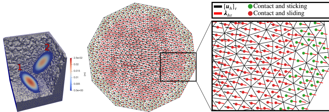
FIGURE 7 Results from Example 2 using approximately 250 000 degrees of freedom. Left: Displacement jump \|[\mathbf{u}_h]\| for the two fractures indicated by the fracture number. Parts of the 3D mesh are cropped to reveal the fractures. Middle: The surface mesh of \Gamma^+ of Fracture 1. The red lines show the tangential part of the Lagrange multiplier \lambda_{h\tau} while the black lines show the scaled displacement jumps 400[\mathbf{u}_h]_\tau . Right: Zoomed view of middle figure
