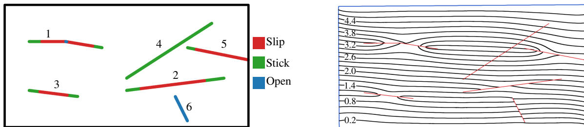
FIGURE 3 The fractured domain from Example 1. Left: The black box corresponds to the domain boundaries, while the fractures, labeled by a number, are represented by lines. The fractures are colored in three colors: segments that slip are red, segments that stick are green, and segments that open are blue. Right: Contour plot of the x -component of the displacement \mathbf{u} . The labels on the contours are given in millimeters. The red lines represent the fractures
