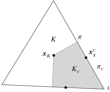
FIGURE 2 Notation used to describe the mesh. For a cell K , face \pi , and vertex v of the mesh, we associate a subcell (K, v) and subface (\pi, v) , as well as a cell center \mathbf{x}_K and continuity point \mathbf{x}_\pi^v . In this figure, the cell is the full triangle, and the subcell is given by the gray area
