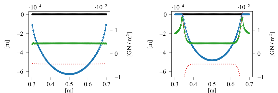
FIGURE A1 The shear component \lambda_r (green), friction bound \pm F\lambda_n (red dashes), tangential displacement jump [\mathbf{u}]_r (blue), and normal displacement jump [\mathbf{u}]_n (black) for the fracture. The dots correspond to the face-centered values. Left: Constant friction coefficient. Right: Regularized coefficient
