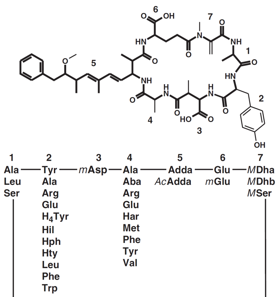
Figure 5. Molecular structure of microcystin-LA together with a schematic of the general structure of possible microcystin peptides. Microcystin-LA differs from microcystin-LR with the substitution of alanine in place of the arginine. ADDA (3-amino-9-methoxy-2,6,8-trimethyl-10-phenyldeca-4,6-dienoic acid) represents a non-protein amino acid side chain present in all microcystin congeners. Molecular structure from Botes et al., 1984 adapted with added schematic by Welker and von Döhren, 2006.
