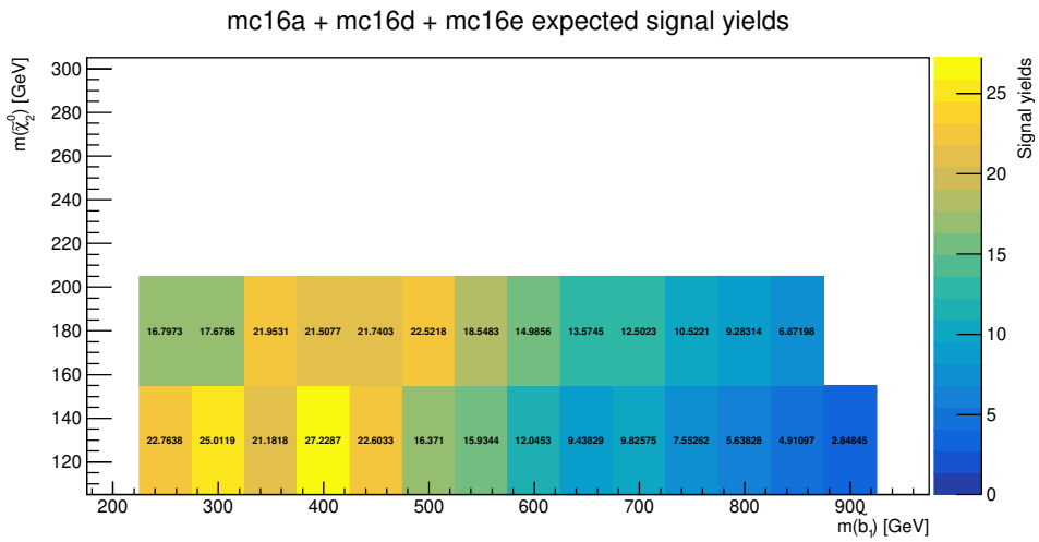
Figure 7.6: Expected signal yields and Asimov significance in the single-bin SR with all cuts applied.
