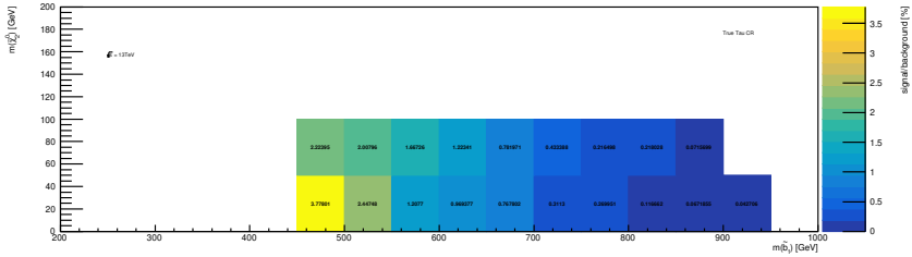
(a) True Tau CR signal contamination
