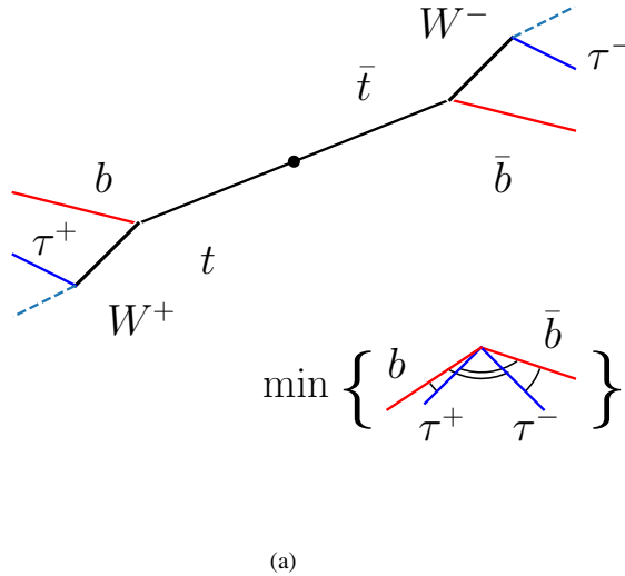
Figure 7.2: Schematic illustration of the \min_{\Theta} variable for a t\bar{t} event.
