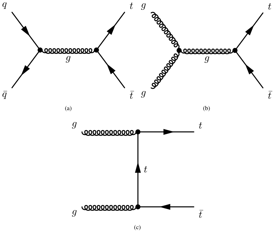
Figure 5.1: Feynman diagrams of t\bar{t} production.
