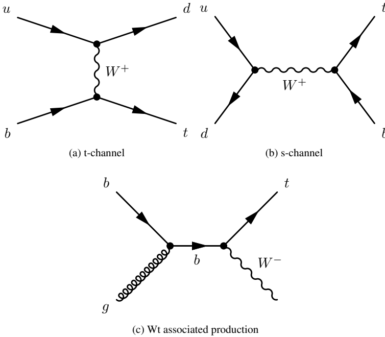
Figure 5.3: Feynman diagrams of single top production.
