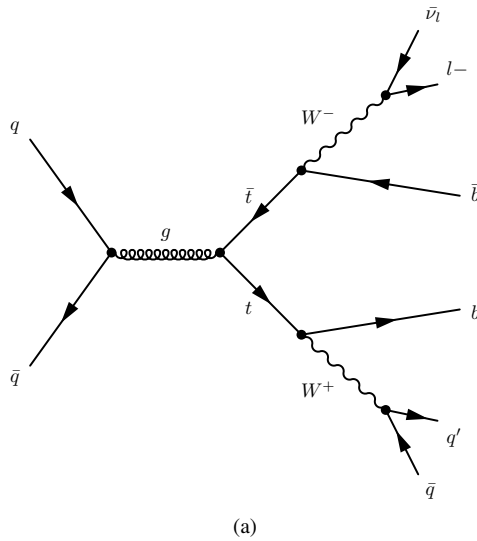
Figure 5.2: An example of semi-leptonic decay of t\bar{t} .
