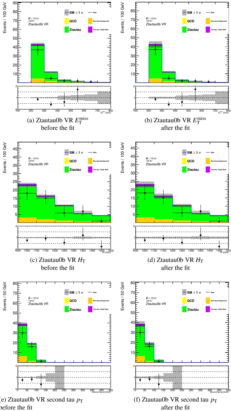
Figure C.1: Distributions of various variables in the Ztautau0b VR before and after the fit. All uncertainties are included and shown as the hatched band. The upper panels show distributions of the expected SM backgrounds with data overlaid. The lower panels show data/MC ratios. In the plots marked "after the fit" the SM backgrounds are scaled with the weights obtained in the background-only fit.
