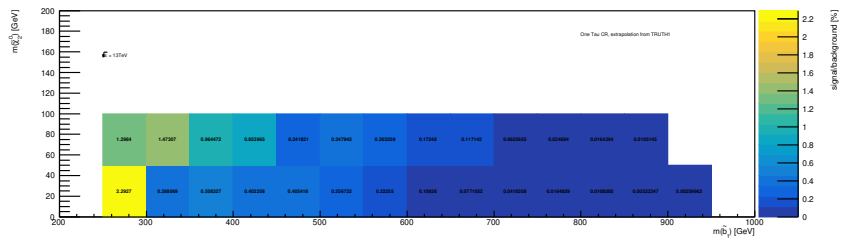
(b) One Tau VR signal contamination extrapolated
