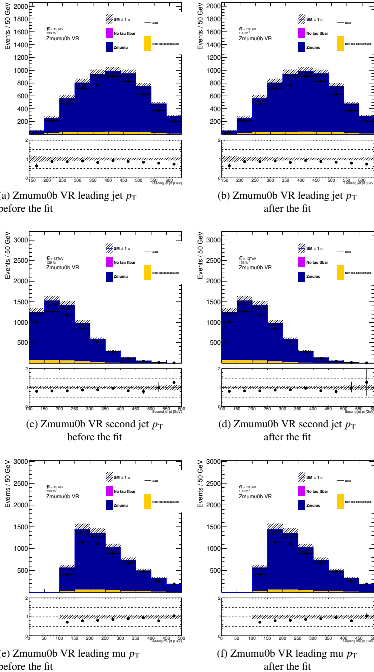
Figure C.4: Distributions of various variables in the Zmumu0b VR before and after the fit. All uncertainties are included and shown as the hatched band. The upper panels show distributions of the expected SM backgrounds with data overlaid. The lower panels show data/MC ratios. In the plots marked "after the fit" the SM backgrounds are scaled with the weights obtained in the background-only fit.
