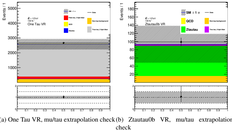
Figure 8.25: Tau VRs with background expectation estimated from muon VRs \times mu/tau extrapolation factor. All uncertainties are included and shown as the hatched band. The upper panels show distributions of the expected SM backgrounds with data overlaid. The lower panels show data/MC ratios. The SM backgrounds are scaled with the weights obtained in the background-only fit.
