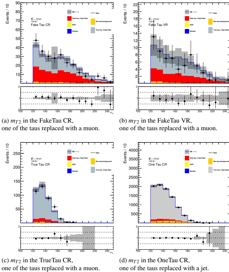
Figure 8.21: Plots of m_{T2} in various regions. All uncertainties are included and shown as the hatched band. The upper panels show distributions of the expected SM backgrounds with data overlaid. The lower panels show data/MC ratios. The SM backgrounds are scaled with the weights obtained in the background-only fit.
