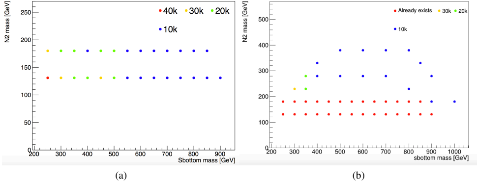
Figure 5.7: Grid points corresponding to different m_{\bar{b}} and m_{\chi_2^0} masses used in the analysis. The colours represent the number of raw Monte-Carlo events produced per data-taking period (mc16a/d/e). (a) shows the initial models considered by the analysis (b) shows the extension of the signal grid.
