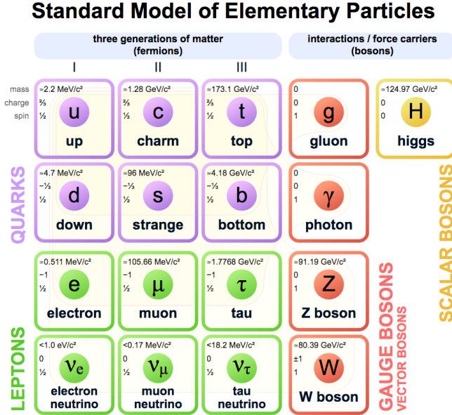
(a) Table of particles of Standard Model [10]. The mass measurements are the latest available as of 2019.
