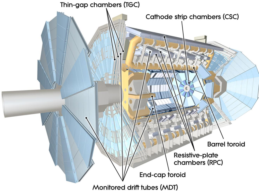
(a) Muon system at the ATLAS experiment. [42]
