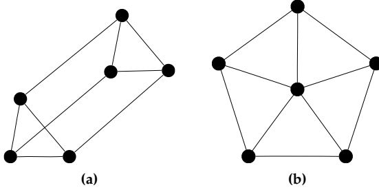
Fig. 1: Two Graph Representations of the Hexacode
