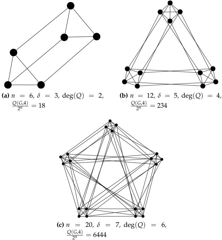
Fig. 7: Examples of Nested Clique Graphs
