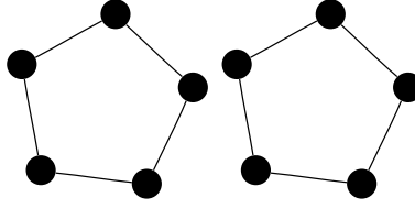
Fig. 3: The “Double 5-Cycle” Graph
