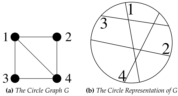
Fig. 3: Example of a Circle Graph
