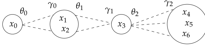
Fig. 4: Example of Construction with PAR_{HN} \leq 8
