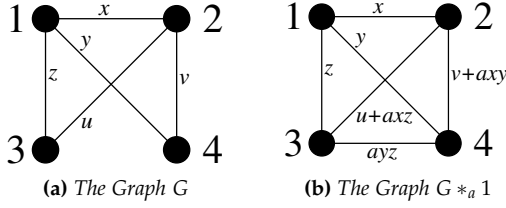
Fig. 3: Example of Generalized Local Complementation
