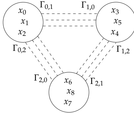
Fig. 6: Example of Construction with Low PAR_{IHN}
