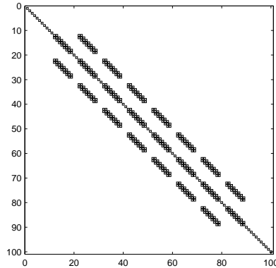
Figure 2.15: Shows the elements in a system matrix for a 8 \times 8 , ghost cells are included.
