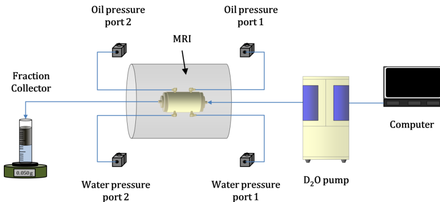
Figure 15: Schematic showing the experimental setup with phase specific pressure ports during the in situ dynamics experiments.
