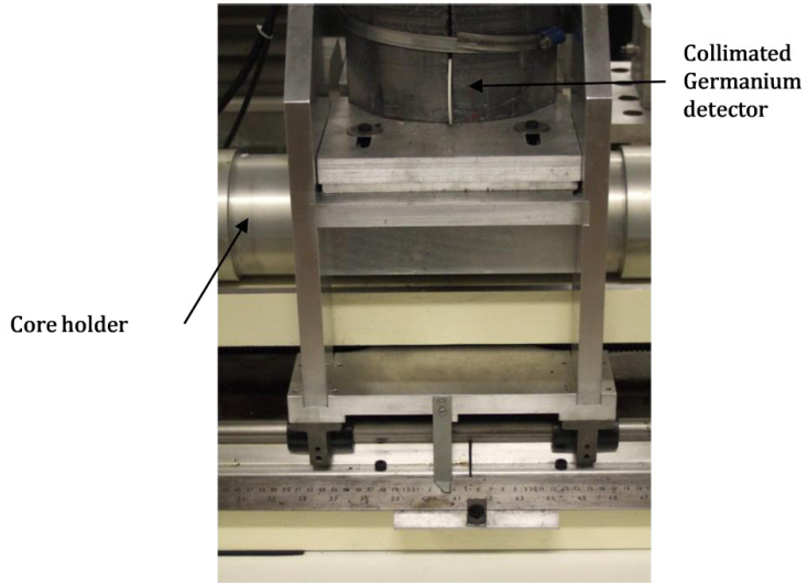
Figure 13: A Germanium detector is positioned above the core holder to obtain the number of \gamma -emissions from segments of the core.
