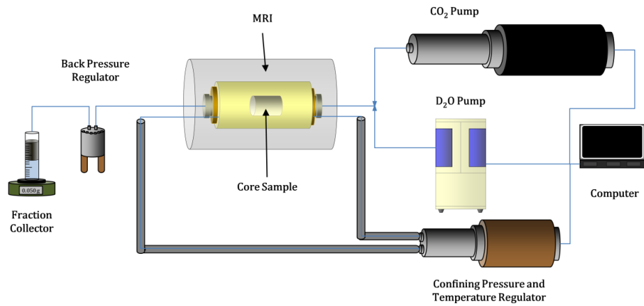
Figure 17: Schematic showing the setup for CO 2 experiments.
