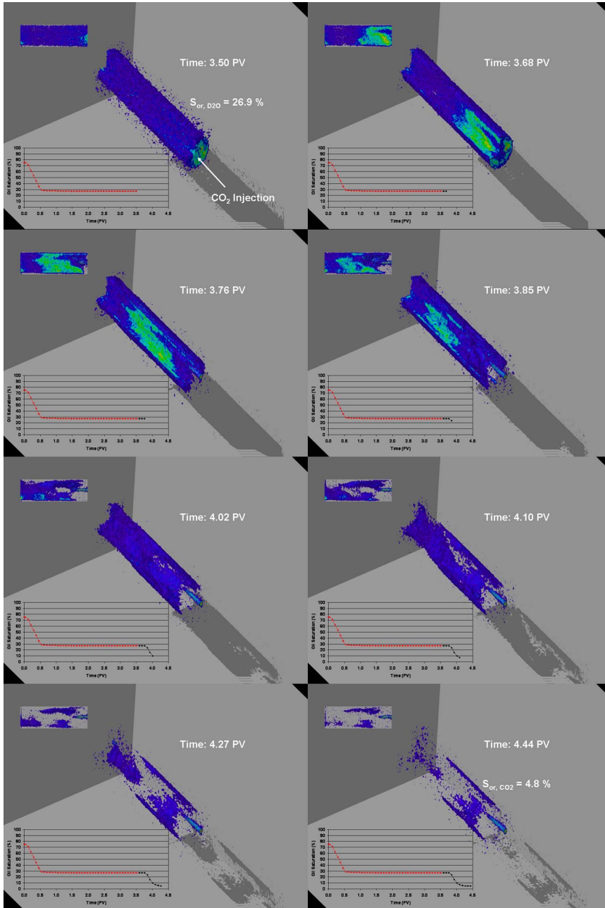
Figure 23: A series of MRI images obtained during injection of CO 2 . A high intensity area advances through the core and leaves only a minimum of detectable signal left.
