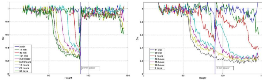
Figure 21: Water saturation distributions in vertically stacked, strongly water-wet sandstone during gravity drainage with an open fracture (left) and with the fracture packed with crushed chalk (right). Capillary continuity was obtained (right), and the volume of the wetting phase otherwise captured by the capillary end effect was produced.
