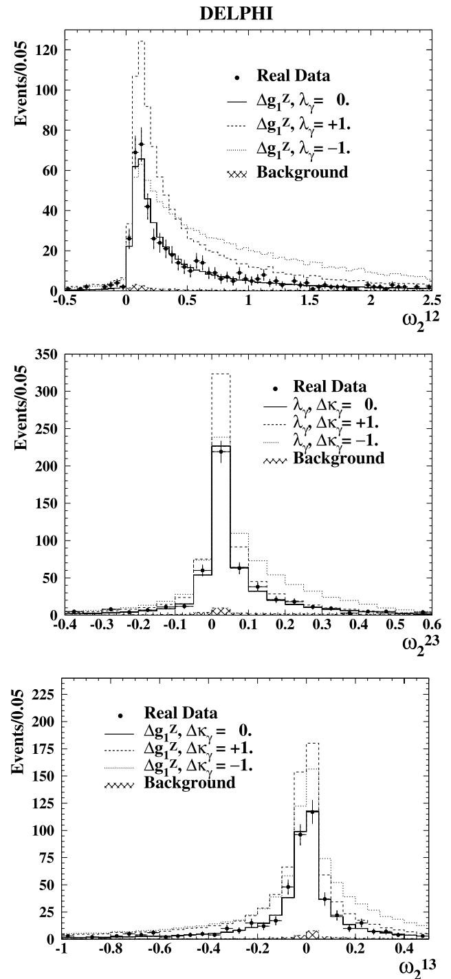
Fig. 5 Distribution of the Optimal Variables \omega_2^{12} , \omega_2^{23} and \omega_2^{13} (the coefficients, respectively, of \Delta g_1^Z \cdot \lambda_\gamma , \lambda_\gamma \cdot \Delta\kappa_\gamma and \Delta g_1^Z \cdot \Delta\kappa_\gamma in the expansion of the differential cross-section in terms of Optimal Variables) for semi-leptonic data at 200 GeV. The points represent the real data, the solid lines the expected distributions for SM values of the couplings, and the dashed lines the expected distributions for the non-SM values of the couplings shown in the legends . The shaded area represents the background. The simulated distributions are normalised to the same luminosity as the data
