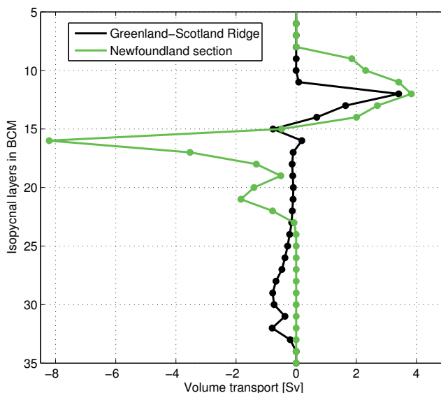
Fig. 13 Net volume transport in density space (represented by the isopycnal layers in BCM) across specific sections, as denoted in the legend. The transports also include the mixed layer transport, which is non-isopycnic. The distribution of the mixed layer transport in density space at the Greenland-Scotland Ridge can be seen in Fig. 5
