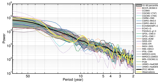
Figure 2: a) The annual mean AMO index in the different models (thin lines) and observations (thick yellow line) relative to the mean of 1901–80. The black thick line shows the ensemble mean and the gray band shows the 10–90 percentile of the model spread. All curves are filtered by a 15 year running binomial filter. The units are given in °C. b) Smoothed power spectrum of the monthly mean AMO. The linear trends are removed and the time series are normalized for different models prior to the analysis. The colours are the same as in (a)
