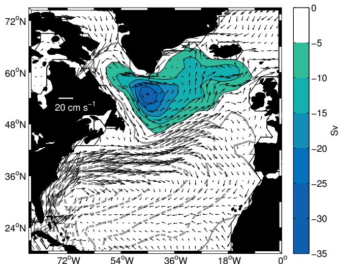
Fig. 3 Mean barotropic streamfunction (contours) with 5 Sv intervals, where filled contours indicate negative and dashed lines indicate positive values. Mean mixed layer velocities are shown by black arrows, with a reference velocity of 20 \text{ cm s}^{-1}
