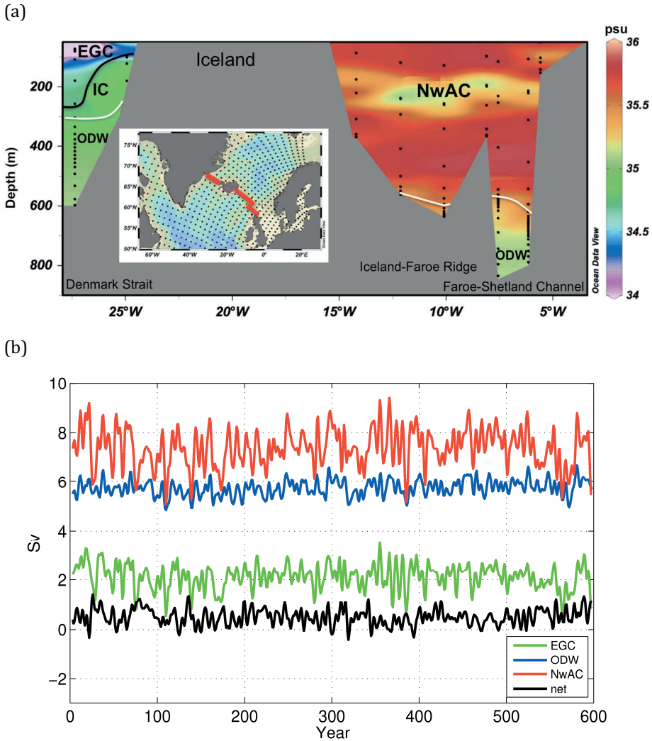
Fig. 8 (a) Cross section of the Greenland-Scotland Ridge, where the salinity is shown in colours. The black line shows the salinity criteria dividing the southward flowing East Greenland Current (EGC) from the northward flowing Irminger Current (IC), which is included in the definition of the Norwegian Atlantic Current (NwAC). White line is the density line dividing the upper flow from the deep overflows (ODW). (b) Low-pass filtered annual volume transports (in Sv) across the ridge. Positive net flow indicates southward flow, where the northward flowing NwAC is weaker than the sum of the southward flowing (EGC and ODW)
