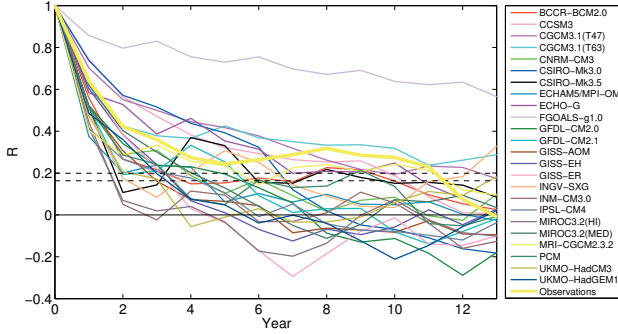
Figure 3: Autocorrelation function for the annual mean values of the AMO index in the different models (thin coloured lines), and for the observations (thick yellow line) to estimate the persistence in the time series. Significance level varies between the two dashed black lines, depending on length of the time series
