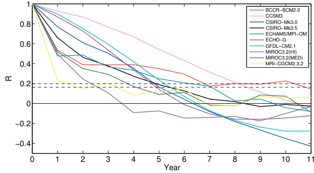
Figure 7: Autocorrelation function for the annual values of AMOC in the different models (coloured lines). Significance level varies between the two dashed black lines, depending on length of the time series. Only the 10 models having a mean overturning within the observed range are shown
