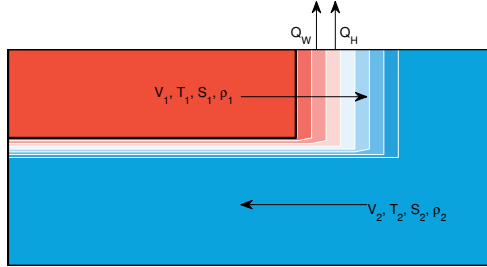
Figure 11: Simple model of the North Atlantic overturning circulation. The red region shows the reservoir simulating the warm tropical and subtropical water with the properties T_1 , S_1 and \rho_1 being transported into the SPG region by the volume transport V_1 . Here the water properties change due to surface cooling and the water sinks and returns as a deep return flow with a volume transport V_2 and the properties T_2 , S_2 and \rho_2 in the blue box. Q_W and Q_H are the net atmospheric freshwater and heat fluxes, defined positive upwards
