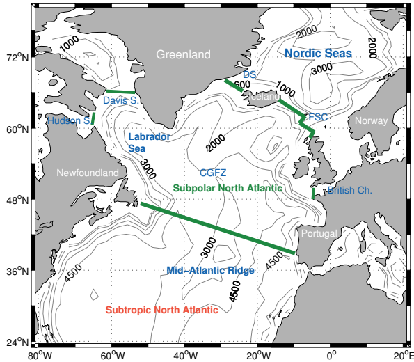
Fig. 1 The model bathymetry (m) of the North Atlantic Ocean and Nordic Seas, with names that are referred to in the text. Abbreviations are: Denmark Strait (DS); Faroe-Shetland Channel (FSC); Charlie Gibbs Fracture Zone (CGFZ). The green sections enclose the subpolar region
