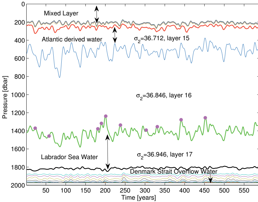
Fig. 8 Time series for the depth (dbar) of the layer interfaces averaged over the Labrador Sea. Black arrows indicate layer thickness. The \sigma_2 -value is given for some of the layers. The magenta dots show end of NAO+ periods > 1.5 std of the filtered normalized time series
