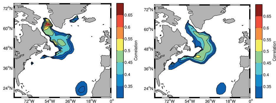
Fig. 10 Correlation between Subpolar Gyre (SPG) strength and anomalies in the layer thickness of the Labrador Sea Water (as indicated in Fig. 8) at SPG maximum (left panel) and 5 years after SPG maximum (right panel)
