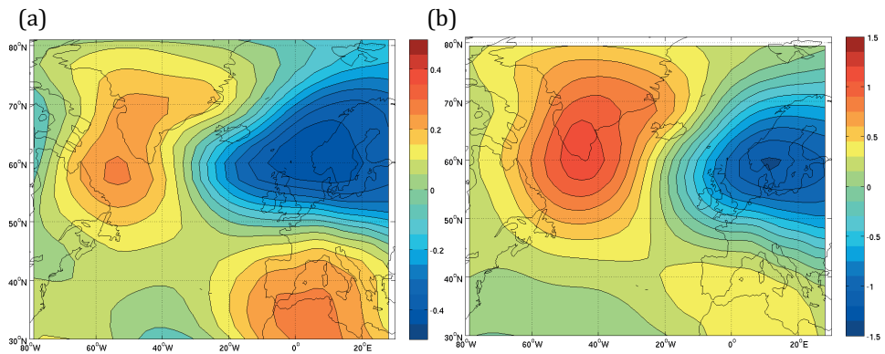
Fig. 13 (a) Correlation between the annual poleward heat transport at the Greenland-Scotland Ridge and the sea level pressure (SLP), where SLP leads by one year (b) negative of EOF3 of the SLP (in hPa \text{std}^{-1} ), also called the Scandinavian Pattern
