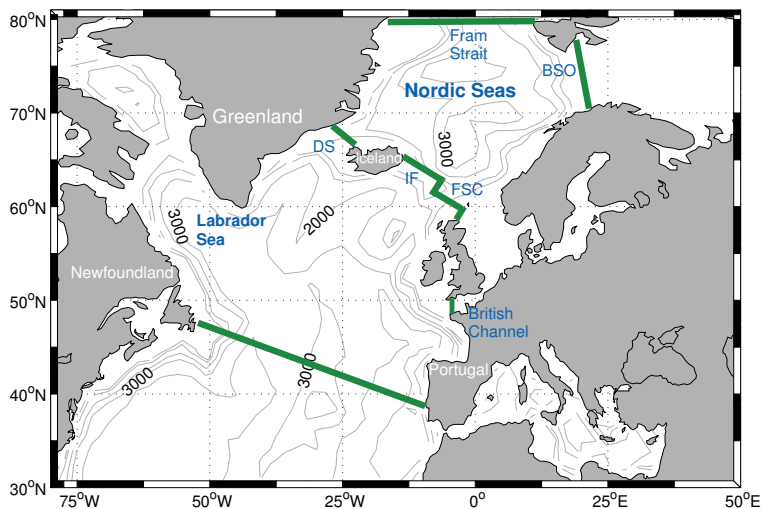
Fig. 1 Bathymetry of the North Atlantic – Nordic Seas region. Green sections show the Fram strait, Barents Sea opening (BSO), the Greenland-Scotland Ridge (GSR) and the British Channel enclosing the Nordic Seas, and the Newfoundland section in the North Atlantic. Openings on the GSR are indicated by the Denmark Strait (DS), Iceland-Faroe Ridge (IF) and Faroe-Shetland Channel (FSC)
