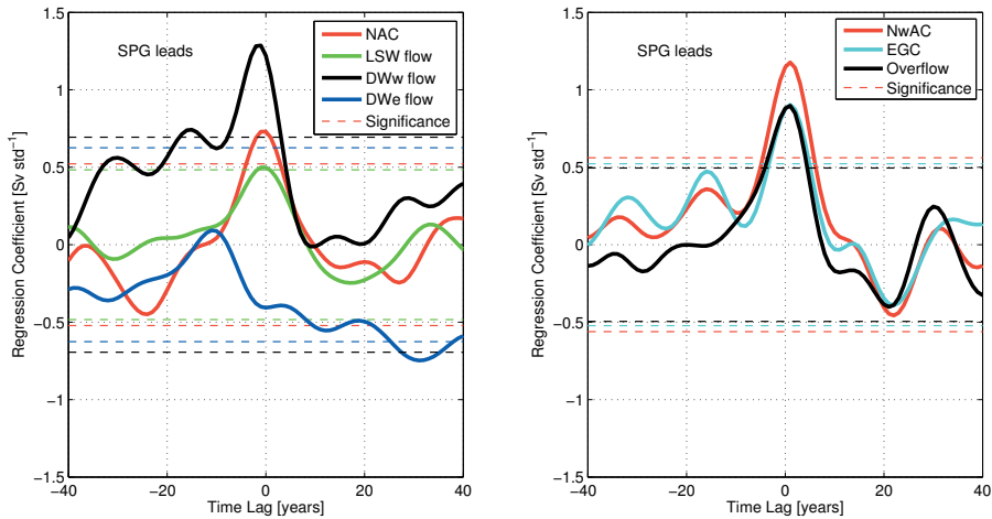
Fig. 6 Subpolar Gyre (SPG) strength regressed on the strength of the different flows across the Newfoundland section (left) and the Greenland-Scotland Ridge (right). An increase of one standard deviation (std) for the DWw flow is associated with an enhancement of the SPG of 1.3 Sv, which is more than a half std of the SPG strength (1 std = 2 Sv). The abbreviations are as given in Table 2.
