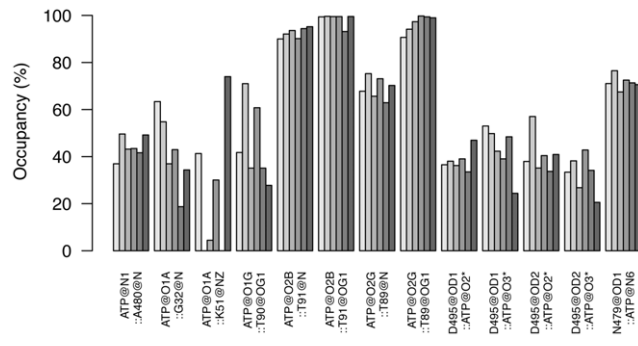
Figure 5. Schematic representation of potential hydrogen bonds between protein and nucleotide. Hydrogen bond donors and acceptors are labeled below the bars in which the height represents the occupancy in % of the simulation time. Each bar depicts the occupancy of one H-bond in one of the 6 ATP-bound simulations (simulations K-P in Figure 2). doi:10.1371/journal.pcbi.1002004.g005
