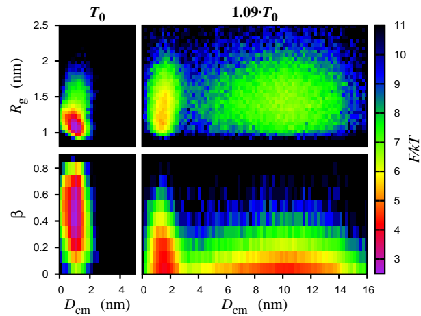
Figure S1. Free energies of binding for A \beta 42 E22G at T_0 and 1.09 T_0 . Symbols are as in Fig. 1.
