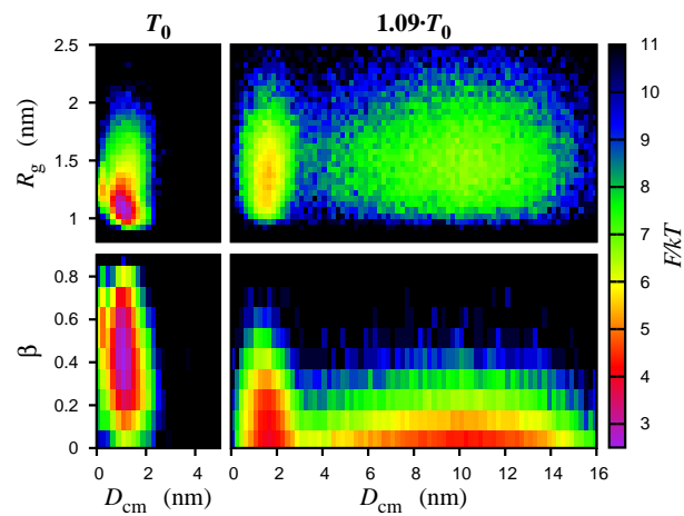
Figure S2. Free energies of binding for A \beta 42 E22G/I31E at T_0 and 1.09 T_0 . Symbols are as in Fig. 1.
