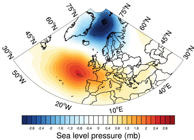
Figure 6. Linear regression of DJF mean sea level pressure anomaly on the gyre index. Regions with 95 % statistical significance are dotted.
