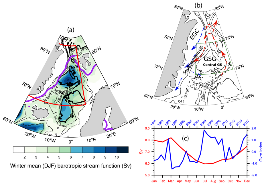
Figure 1. (a) Winter-mean (DJF) barotropic stream function for the period 1991–2017. The region marked in red indicates the Nordic Sea region. The purple line shows the mean DJF sea ice extent for the study period. (b) Schematic of the major currents discussed in the text. JMC: Jan Mayen Current; EGC: East Greenland Current; GSG: Greenland Sea Gyre. Warm currents are drawn in red, and cold currents are in blue. Black contours show bottom topography drawn every 1000 m. The thick black contour indicates the 3000 m isobath. The marked region in dark green is used to calculate the “gyre index” as detailed in the next section. (c) The blue line indicates the gyre index used in this study, and the red line shows the annual cycle of the strength of GSG circulation determined by averaging barotropic stream function within the 3000 m isobath in the region marked in (b).
