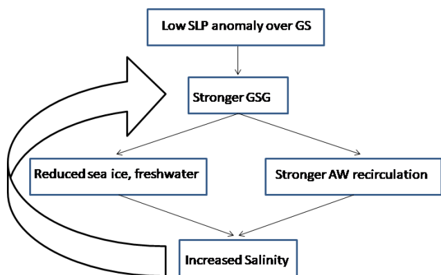
Figure 13. A proposed positive oceanic feedback induced by atmospheric forcing in NS.
