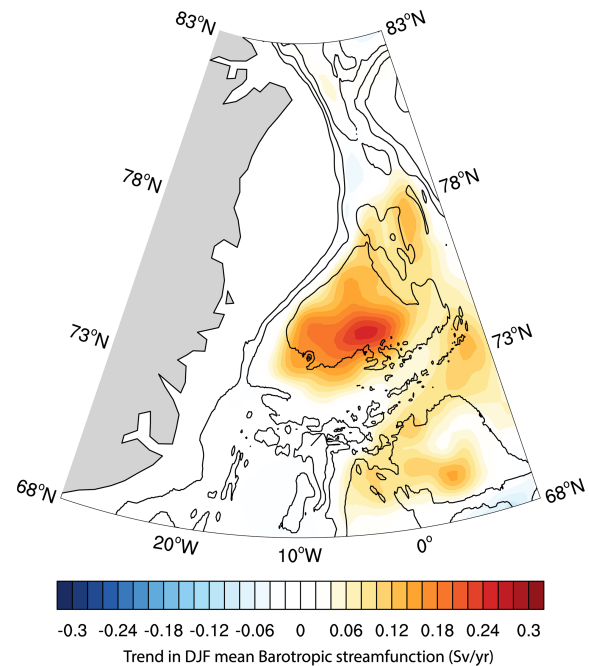
Figure 12. Linear trend ( \text{Sv yr}^{-1} ) in winter-mean (DJF) barotropic stream function for 1991–2017. Only significant values at the 95 % level are shown for clarity. Contours are bottom topography drawn every 1000 m.
