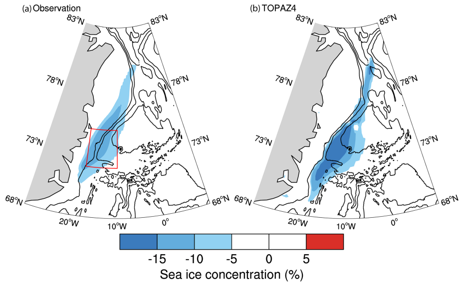
Figure 5. Linear regression of winter-mean (DJF) sea ice concentration from (a) satellite observations and (b) TOPAZ4 reanalysis on the gyre index. Only significant values at the 95 % level are shown. Contours are bottom topography drawn every 1000 m.
