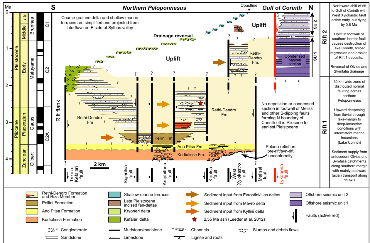
Fig. 9. N-S swath chronostratigraphic section showing proposed age-model and provenance for the central onshore Corinth rift together with correlation with offshore (based on Nixon et al. , 2016). Location in space and time of lithology and sedimentary bodies shows present-day preservation and exposure of the various units. Details of present erosion level omitted for clarity. Faults are named along bottom of diagram. See text for full discussion.
