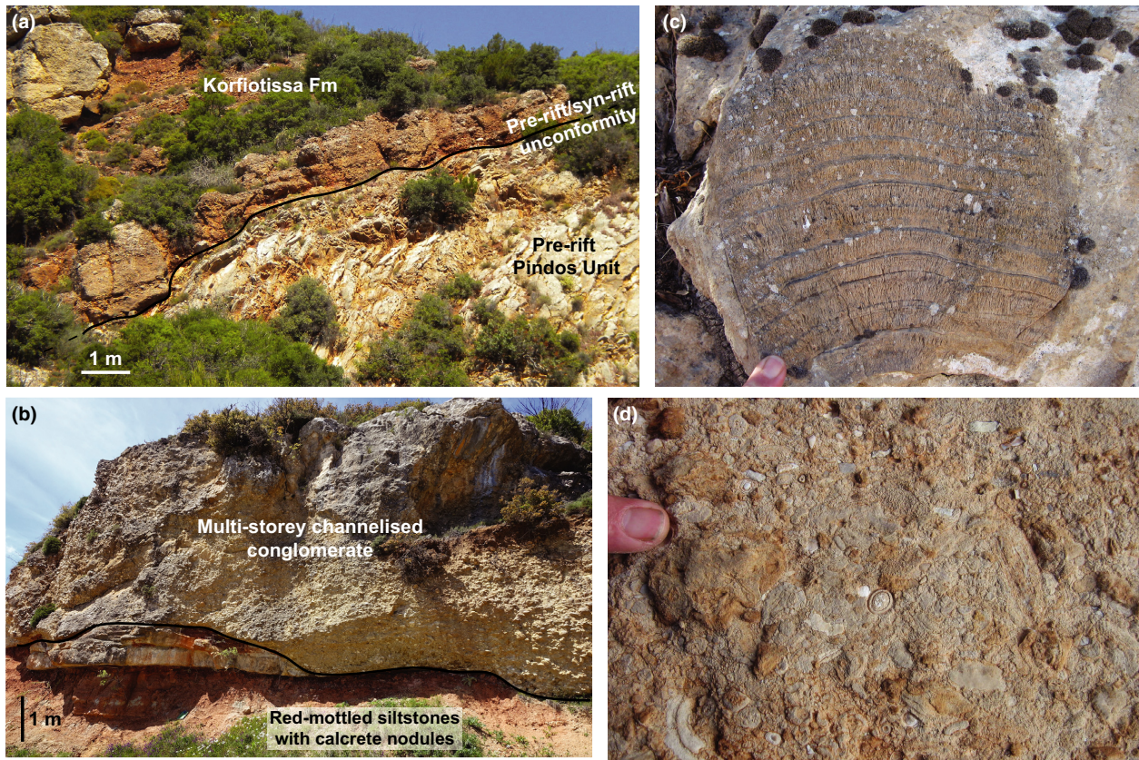
Fig. 4. Sedimentary characteristics of the Korfiotissa and Ano Pitsa formations (see Fig. 2 for location). (a) Basal unconformity with onlapping conglomerates of the Korfiotissa Formation, west flank of the Fonissa gorge, Xylokastro horst (0635778 4215838). (b) Example of fluvial channelized conglomerate facies association eroding into floodplain, intercalated sandstones and mudstones facies association, Korfiotissa Formation (0633503 4214660). (c) Block of freshwater marly limestones containing reworked seasonally banded tufa within Ano Pitsa Formation. The tufa blocks were probably eroded during high fluvial discharge from nearby palustrine marginal springs mounds, Xylokastro horst (0632590 4216336). (d) Detrital tufa fragments and pisoids in coarse-grained basal part of bedded detrital freshwater limestones with low angle cross-bedding, interpreted as lake margin environment. Ano Pitsa Formation, Xylokastro horst (0632590 4216336).
