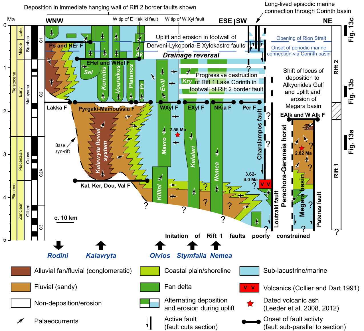
Fig. 12. The WNW-ESE to NE-SW swath chronostratigraphic section along the northern Peloponnese and Corinth and Megara basins. Details of footwall erosion and terraces are omitted for clarity. Location of major drainage catchments shown with block arrows at base of figure. Western rift is modified after Ford et al. (2016) and Hemelsdaël et al. (2017); central rift – this study and Leeder et al. (2012); Corinth basin based on Collier & Dart (1991) and Megara basin after Bentham et al. (1991) and Leeder et al. (2008). Delta abbreviations – Ak, Akrata; Ev/II, Evrostini/Ilias; Kry, Kryoneri; Pr, Prioni; Sel, Selinous. Selected fault names in bold; abbreviations – EAlk and WAlk F, East and West Alkyonides faults; EHel and WHel F, East and West Heliki faults; EXyl F, East Xylokaastro fault; Kal, Ker, Dou, Val F, Kalavryta, Kerpini, Doumena and Valimi faults; NKia F, North Kiato fault; Per F, Perachora fault; Ps and NEr F, Psathopyrgos and Neo Erineos faults; WXyl F, West Xylokaastro fault.
