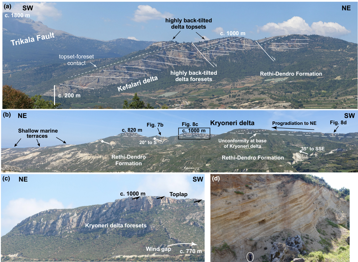
Fig. 8. Coarse-grained deltas and marine terraces (see Fig. 2 for location). (a) West side of the northern Stymfalia valley NE of the town of Kefalari. Topsets and foresets of the Kefalari delta are highly rotated (to S) in the hanging wall of the Trikala-Kefalari Fault. The hills to the SW are composed of pre-rift Hellenide units in the footwall of the Trikala Fault. (b) Coarse-grained Kryoneri delta unconformably overlying S- to SE-tilted Rethi-Dendro Formation along the E side of Sythas Valley. Note strongly progradational character of the Kryoneri delta capping the valley sides and shallow marine terraces at lower elevation (left of photo). (c) View of stratal geometry within the Kryoneri delta. Note lack of topsets and strongly progradational character. The top of the delta is a sub-horizontal topset surface which is itself incised (edge of incised valley [now a wind gap] just visible on right of photo). Main cliff is approximately 200 m high; location shown in (b). (d) Detail of foreset facies within the Kryoneri delta showing open-framework, clast-supported conglomerates with lenticular to lobate bedding geometry, dipping at up to 30°. Person circled for scale; location shown in (b).
