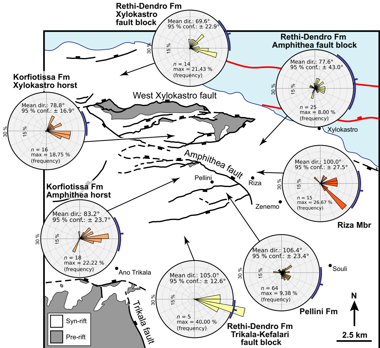
Fig. 5. Summary of palaeocurrent data from the Korfiotissa, Pellini and Rethi-Dendro formations for different structural domains within the study area. Simplified geological map with pre-rift Hellenide basement and syn-rift shown. Faults active post 0.8 Ma – red; older, inactive faults – black.
