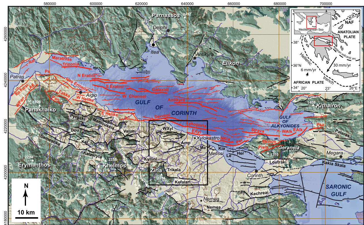
Fig. 1. General topography and geology of the Corinth rift. Pre-rift Hellenide basement (green), Plio-Pleistocene syn-rift sediments (tan) and main normal faults (faults active post 0.8 Ma – red; older, inactive faults – black). Contour interval = 500 m. Location of detailed central, onshore study area of Fig. 2 also shown. Note higher topographic relief north and south of the Gulf of Corinth towards the west. Inset shows study area in the context of Aegean/Mediterranean tectonic boundaries and plate motions. Offshore faults from Nixon et al. (2016); onshore faults from the authors' own mapping and Ford et al. (2013, 2016); Rohais et al. (2007a). Fault names in bold; abbreviations – AK, Ano Kastritsi fault; Amp, Amphithea fault; Dou, Doumena fault; EAlk, East Alkyonides fault; EXyl, East Xylokaastro fault; Her, Heraion fault; Ker, Kerpini fault; Kia, Kiato fault; Le, Lechion fault; Me, Melissi fault; Naf, Nafpakto fault; NKia, North Kiato fault; Pan, Panachaikon fault; Per, Perachora fault; Ps, Psathopyrgos fault; Psa, Psatha fault; WAlk, West Alkyonides fault; WPan, West Panachaikon fault; WXyl, West Xylokaastro fault.
