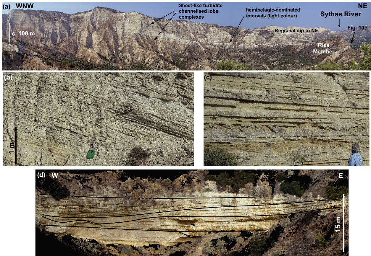
Fig. 7. Sedimentary characteristics of the Rethi-Dendro Formation (see Fig. 2 for location). (a) Large-scale view of the stratigraphy of the formation within the Amphithea fault block (W side of Sythas valley) showing tens of metre, sheet-like alternation of sandstone-rich and marl-dominated facies associations. (b) Marlstone and sandstone facies association (0640370 4209033). (c) Sandstone-dominated facies association with tabular bedded turbidites and thin intraformational slumps (0627472 4219503). (d) Digital outcrop model of channel complex composed of sandstone and conglomerate facies association of the Riza Member with the main erosive boundaries are highlighted. Field of view is 90 m (0638870 4212670). Digital outcrop model is based on a combination of LiDAR and photogrammetry.
