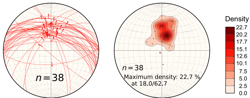
Fig. 10. Summary of fault planes and striations on major exposed normal faults (lower hemisphere, equal area plots). Bottom left – summary of fault dip and fault striation data. Bottom right – density plot of fault striations, indicating mean slip vector 62^\circ to 018^\circ . Plots created with OpenStereo software ( http://www.igc.usp.br/?id=391 ).
