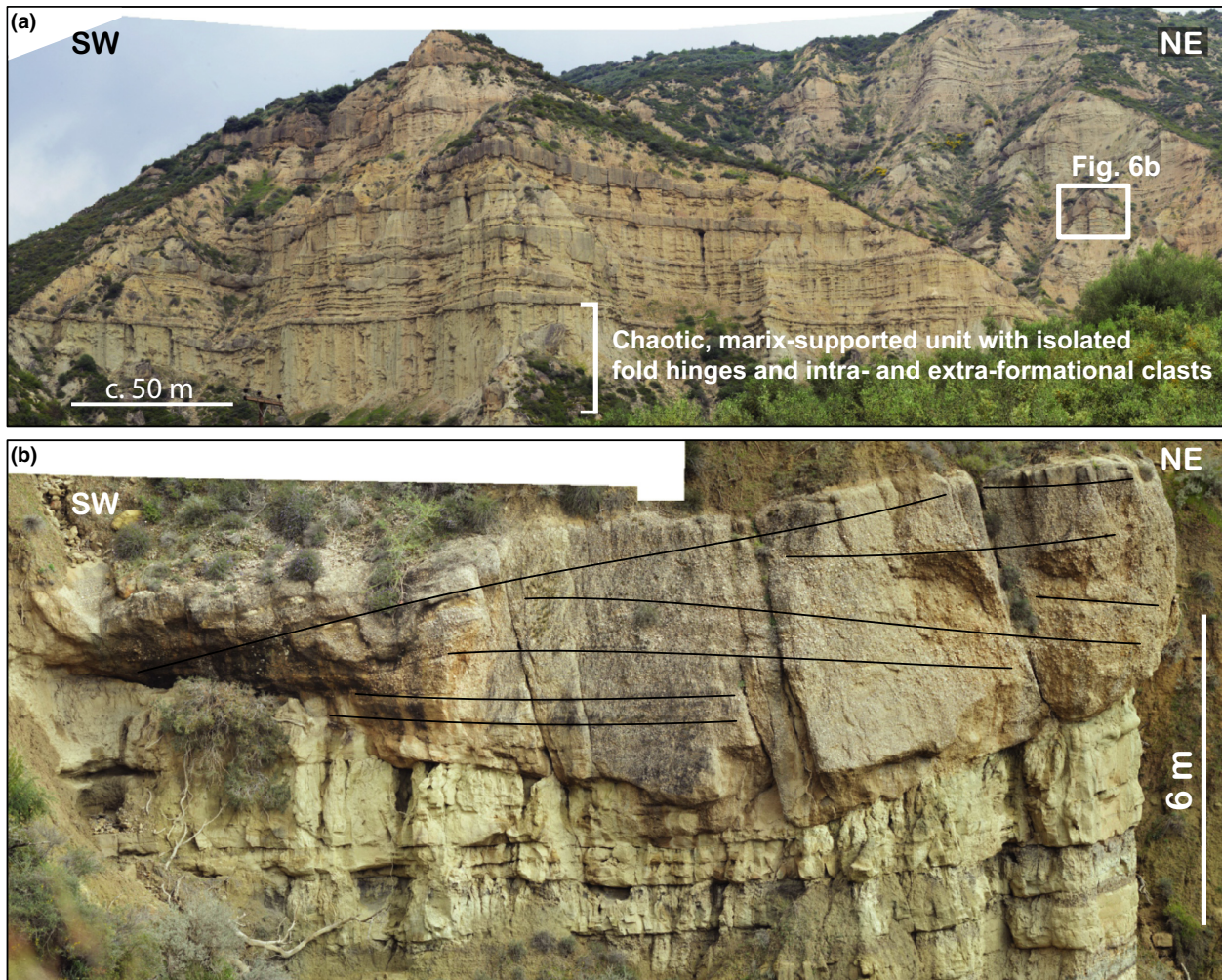
Fig. 6. Sedimentary characteristics of the Pellini Formation (see Fig. 2 for location). (a) Overview showing typical stratigraphic architecture of alternating sheet-like to channelized conglomerates and sandstones, and interbedded mudstones, marlstones and sandstones facies associations. Note the 25 m thick intraclast-dominated and folded unit (mass transport deposit) at the base of the section (0637608 4210588). (b) Detail of channelized conglomerates eroding into a succession of tabular medium to coarse sandstones interbedded with laminated mudstone. The inclined bedding in the conglomerate channel is interpreted to represent lateral accretion surfaces (0637300 4210935).
