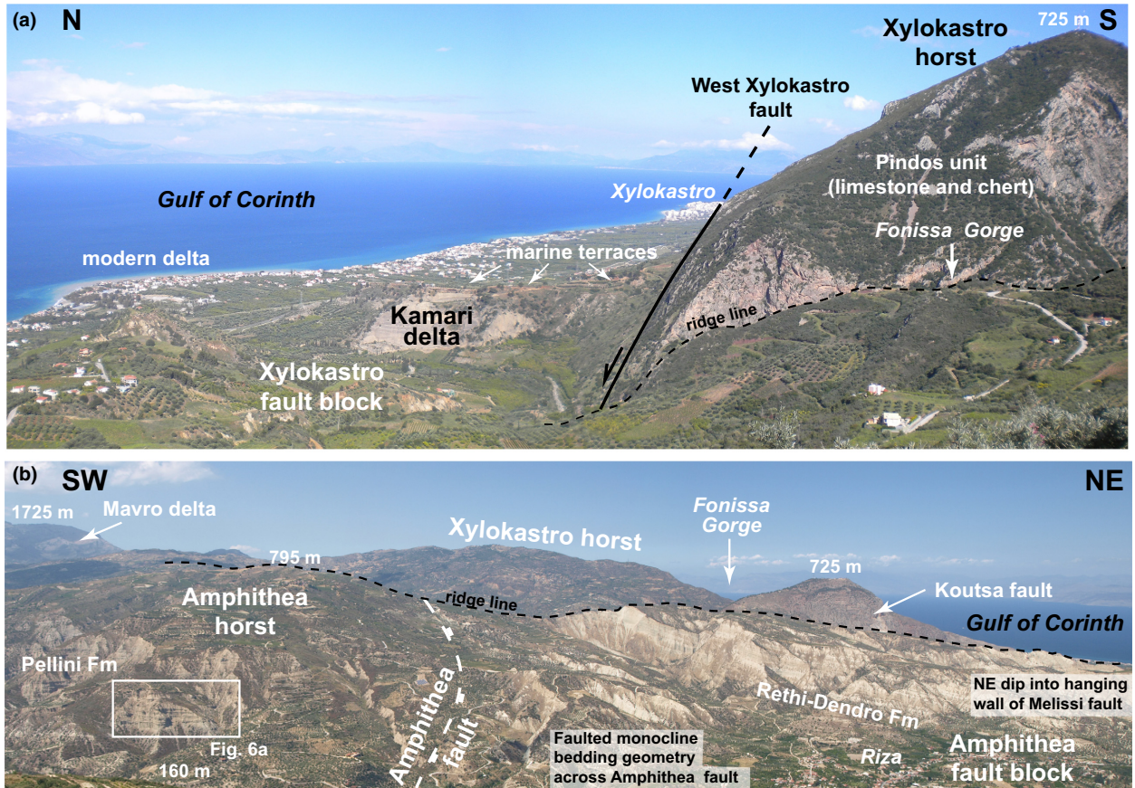
Fig. 11. Structural and stratigraphic relationships from different structural domains within the study area (see Fig. 2 for location). (a) View east along the easternmost segment of the West Xylokaastro fault (Kamariotiko segment) showing Pindos unit limestones and cherts in the footwall (Xylokaastro horst), with Late Pleistocene deltaic (Kamari delta) and shallow marine deposits unconformably overlying Rethi-Dendro Formation (covered) in the hanging wall (Xylokaastro fault block). (b) West side of the Sythas valley overlooking the town of Riza showing monoclonal geometry of bedding in the hanging wall of the Amphithea Fault. The overall NE dip of bedding in the Amphithea fault block, interpreted to be due to syn-depositional tilting into the immediate hanging wall of the S-dipping Melissi Fault. The crest of the Xylokaastro horst forms the skyline and the Mavro delta can be seen on the top left. Sigeritsa and other NE-SW-striking faults are not shown for clarity.
