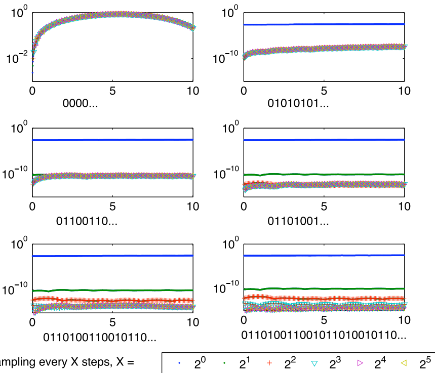
Fig. 1 “Modes” of the symmetry error e_k = \max_{x_i, y_j} |u_k(x_i, y_j) - u_k(y_j, x_i)| versus time t_k = kh for the method of alternating directions for the PDE u_t = u_x + u_y + 2 \times 10^{-3}u^2 , on a square ( L = 1 ), with initial condition u_0 = e^{-x^2 - y^2} , isotropic mesh and periodic boundary conditions. See Example 3.1 for details. The integration is performed using the Forward Euler as a basic method. The order of the overall approximation is the same as the original method (first order only), the only difference is the order of the directions, chosen according to the Thue–Morse sequence. The different symbols correspond to different sampling rates: every step, every second step, fourth, eighth, .... From top left to bottom right: sequences ‘0’, ‘01’, ‘0110’, ‘01101001’, etc.
