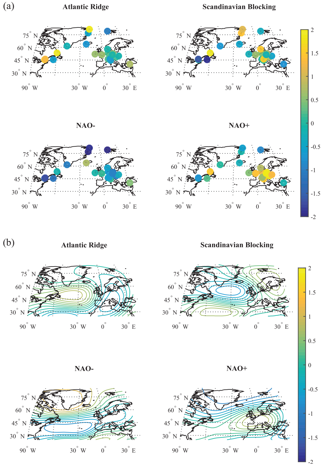
Fig. 1. (a) The composite response of \delta^{18}\text{O} of GNIIP according to the 20CR V2 500 mb gph clustering indices. Colour bar represents normalized (z-scored) values. (b) The North Atlantic weather regimes according to 20CR V2 500 mb gph for the period of 1871–2012. The average z-score values for 11 central European stations (excluding Reykjavik, Svalbard and Ankara) show \delta^{18}\text{O} enrichment for NAO+ (1.25‰) and \delta^{18}\text{O} depletion for NAO– (−0.51‰), indicating a clear \delta^{18}\text{O} response associated with the different phases of NAO. For the Atlantic Ridge, negative anomalies are present over central Europe although the average anomaly is weak (0.05‰) while East N-America shows tendencies towards positive anomalies (two positive stations out of three). The Scandinavian Blocking shows the opposite, where anomalies over central Europe show positive anomalies with an average value of 0.40‰ while on the other side of the North Atlantic two out of three stations show negative anomalies.
