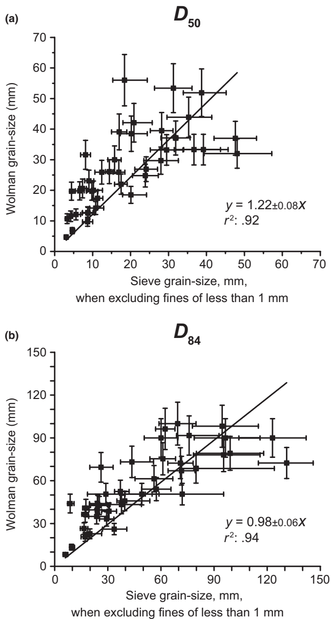
FIGURE 6 (a) Comparison of Wolman point count D_{50} with sieved D_{50} (when excluding fines of less than 1 mm). Wolman point count error bars are \pm 15\% and sieve error bars denote D_{45} – D_{55} . (b) Comparison of Wolman point count D_{84} with sieved D_{84} (when excluding fines of less than 1 mm). Wolman point count error bars are \pm 15\% and sieve error bars denote D_{79} – D_{89}
