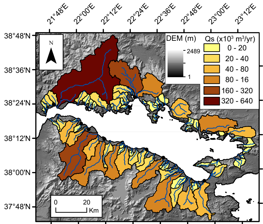
FIGURE 3 BQART modelled annual suspended sediment fluxes from Watkins et al. (2018), scaled by 1.6 to match the Holocene basin volume ( 35 \text{ km}^3 ), to derive the full suspended sediment flux for each catchment
