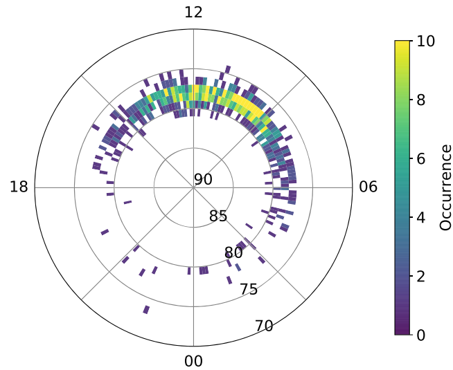
Figure 1. Occurrence distributions in MLAT/MLT coordinates binned into 1° by 2° bins of the flow channel center at the beginning of each event within the study.
