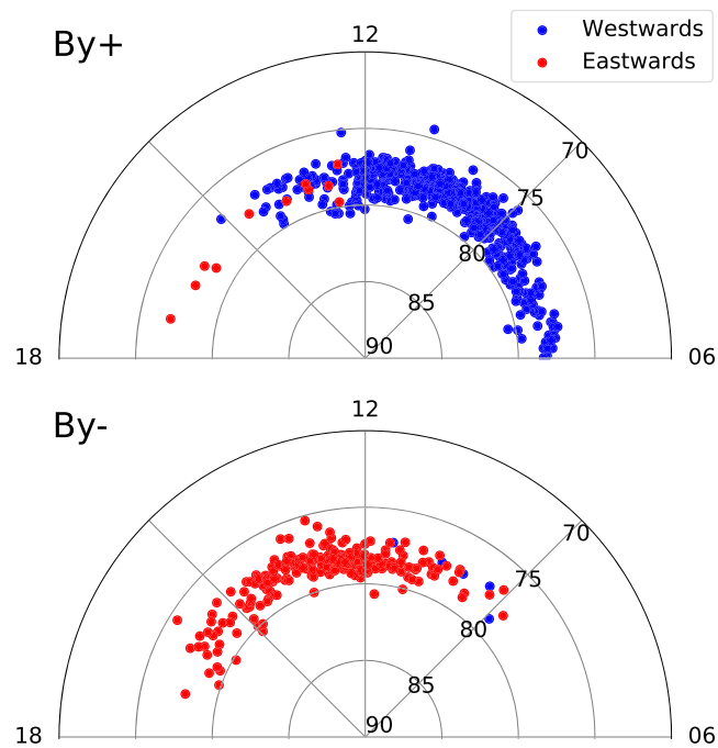
Figure 2. Occurrence distributions in MLAT/MLT coordinates for (top) IMF By+–dominated and (bottom) IMF By–dominated solar wind conditions. Filled circles represent the direction of the plasma flow within the channel center at the beginning of each event, where blue and red indicate flows westward (toward) and eastward (away) from the Longyearbyen radar, respectively.
