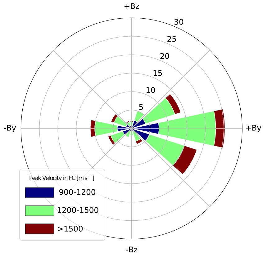
Figure 5. Wind rose diagram showing 30° wide solar wind clock angle radial spokes, colored to peak flow channel velocity magnitudes of 900–1,200 m s -1 (blue), 1,200–1,500 m s -1 (green), and >1,500 m s -1 (red). The radial axis shows the percentage of flow channel occurrence, increasing in 5% increments.
