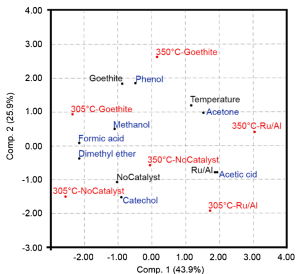
Fig. 6. Biplot containing all the experiments, all variables, and all the identified and quantified compounds from this work.
