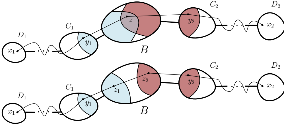
Figure 1: Illustration of the proof of Lemma 3. The top drawing shows item (i) and the bottom one item (ii).
