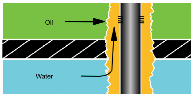
Fig. 2 Flow behind pipe
