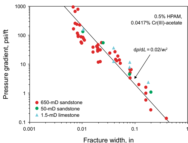
Fig. 18 Pressure gradient for gel extrusion versus fracture width
