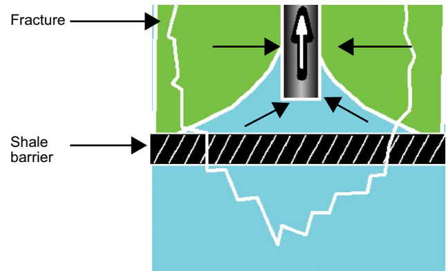
Fig. 7 Fracture leading from a vertical production well down to an aquifer
