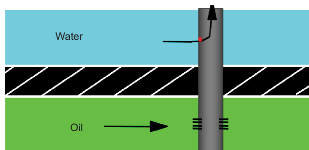
Fig. 3 Casing leak
