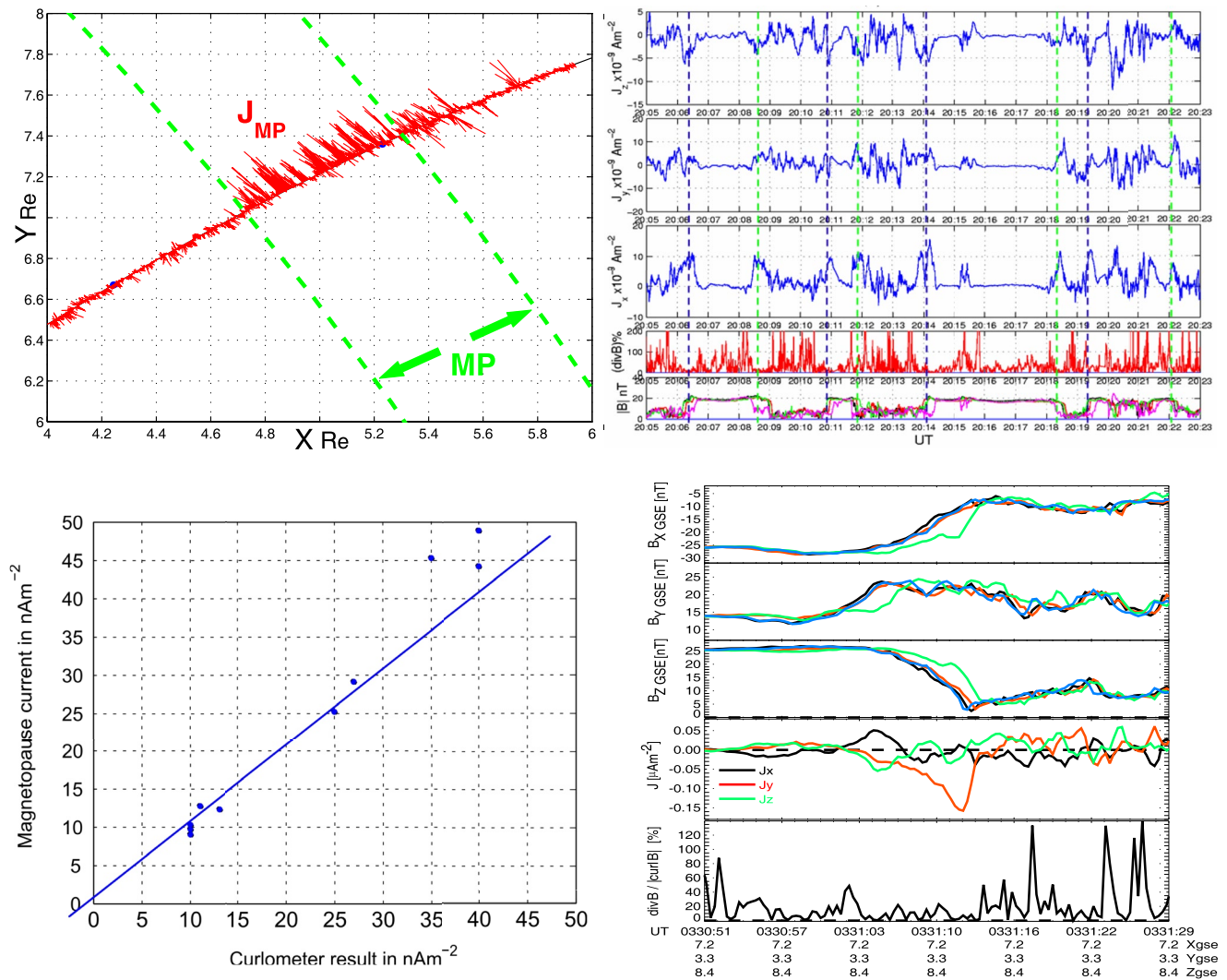
Figure 3. (top left) Projected current density vectors from the Curlometer for the period of repeated MP traversals on the January 26, 2001, as Cluster moves outbound through repeated in-out motions of the MP and into the magnetosheath. (top right) The MP current density, showing changes in orientation which follow the MP orientation during a series of ripples or large scale boundary waves (lower panels are the value of Q and the multi-spacecraft magnetic field magnitude). (bottom left) Comparison of the magnetopause current density estimated from an equivalent Chapman-Ferraro sheet to the curlometer for a range of crossings (from Dunlop & Balogh, 2005). (bottom right) Plot of the multi-spacecraft plasma density, magnetic field and current density, with values of Q at the bottom, for a thin magnetopause (on March 2, 2002), where the spacecraft separation was \sim 100 km. Estimated current densities reach 160 \text{ nAm}^{-2} and calculated from MVAJ as extending over 200 km (from Haaland, Sonnerup, Dunlop, Georgescu, et al., 2004).
