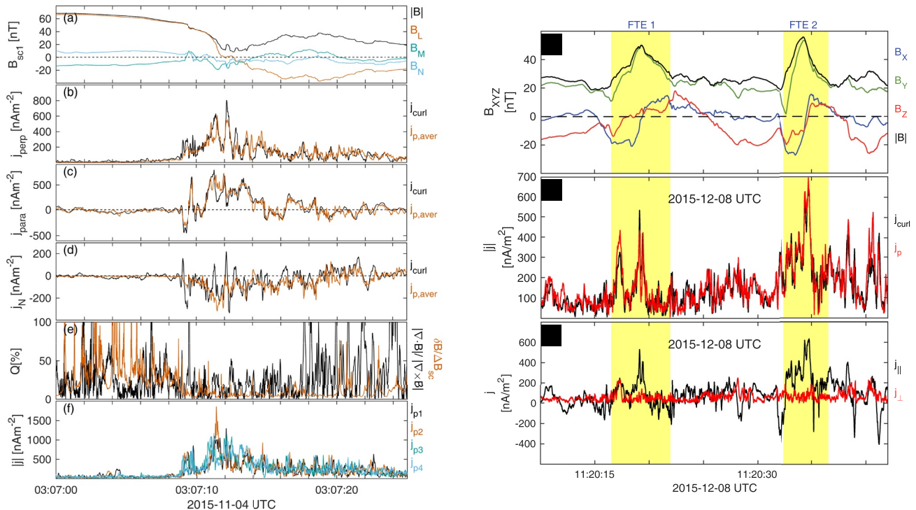
Figure 12. (left) A typical MP crossing for a thickness of \sim 350 \text{ km} seen by MMS, showing: (a) L, M, N coordinates of the magnetic field, (b) to (d) the perpendicular, parallel and normal components of J from the curlometer estimate and the mean value of the 4-spacecraft ion moments, (e) the quality parameter Q compared to a crude (upper) estimate of the measurement errors from \delta B/\Delta B , (f) the individual |i| from the plasma moments at each spacecraft. (right) Detailed current structures of two ion-scale FTEs: (a) magnetic field with bipolar signatures in the normal component ( B_N ) during each FTE interval; (b) A consistent current result from the curlometer and plasma moments, respectively, and (c) Parallel and perpendicular currents (after Dong et al., 2017).
