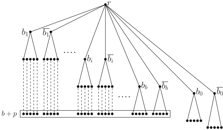
Fig. 4 Figure showing the constructed tree after the first phase
