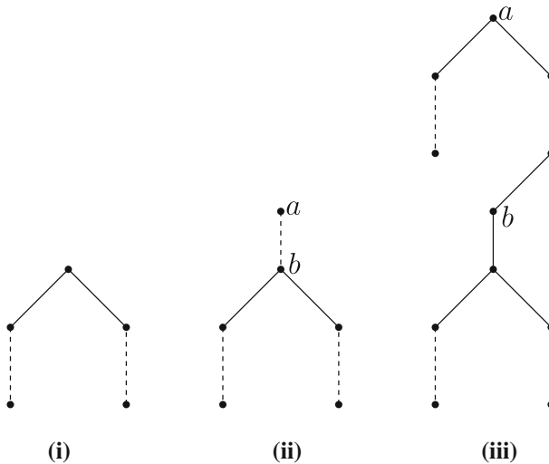
Fig. 3 (i) A ladder tree. (ii) A bell tree. (iii) A snake tree. Dashed segments denote paths
