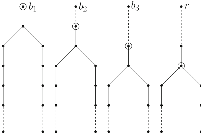
Fig. 5 Figure showing parts of the three snake trees and the bell tree corresponding to the literals of C_j . The circled vertices are selected in the solution
