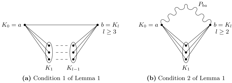
Fig. 1. (a). Condition 1 of Lemma 1: (a, b) \in E_H and l \geq 3 . (b). Condition 2 of Lemma 1: (a, b) \notin E_H and there exists a path P_{ba} from b to a in H[K_l, \dots, K_{p-1}, K_0] .
