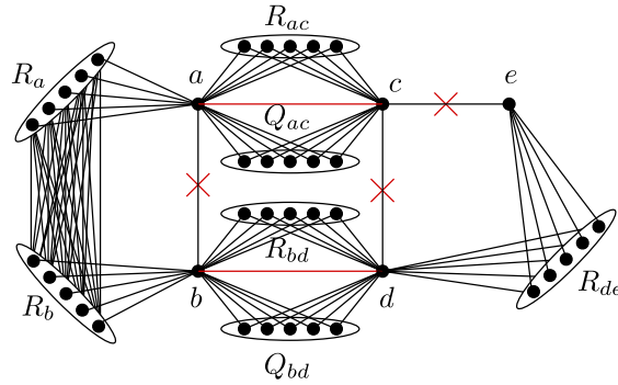
Fig. 5. Graph G_4 is shown in black. Fat cycles \{a\}, R_a, R_b, \{b\} and \{d\}, \{c\}, \{e\}, R_{de} are combined with two fat cycles \{x\}, R_{xy}, \{y\}, Q_{xy} , for x, y = a, c and x, y = b, d . Each of the thick cliques has (n - 5)/7 vertices. When n \geq 26 , G_4 admits a unique minimum editing with the 3 deleted edges and 2 fill edges shown in red.
