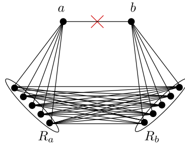
Fig. 3. Graph G_2 is shown in black. It is a fat cycle \{a\}, \{b\}, R_b, R_a . The thick cliques R_a and R_b each have (n - 2)/2 vertices, where n \geq 6 . For x \in R_a and y \in R_b , (x, y) \in E_{G_2} . When n \geq 6 , G_2 admits a unique minimum editing that deletes the edge (a, b) .
