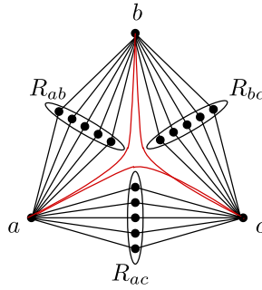
Fig. 2. Graph G_1 is shown in black. It is a fat cycle \{a\}, R_{ab}, \{b\}, R_{bc}, \{c\}, R_{ac} . Each of the thick cliques R_{ab}, R_{bc} , and R_{ac} has (n - 3)/3 vertices. When n \geq 15 , G_1 admits a unique minimum chordal editing that adds the three fill edges shown in red. (For interpretation of the colors in the figure(s), the reader is referred to the web version of this article.)
