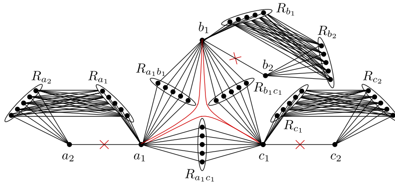
Fig. 4. Graph G_3 is shown in black. The fat cycle \{a_1, R_{a_1b_1}, \{b_1\}, R_{b_1c_1}, \{c_1\}, R_{a_1c_1}\} is combined with three fat cycles \{x_1\}, \{x_2\}, R_{x_2}, R_{x_1} for x \in \{a, b, c\} . Each of the thick cliques has (n - 6)/9 vertices. When n \geq 42 , G_3 admits a unique minimum editing with the 3 deleted edges and 3 fill edges shown in red.
