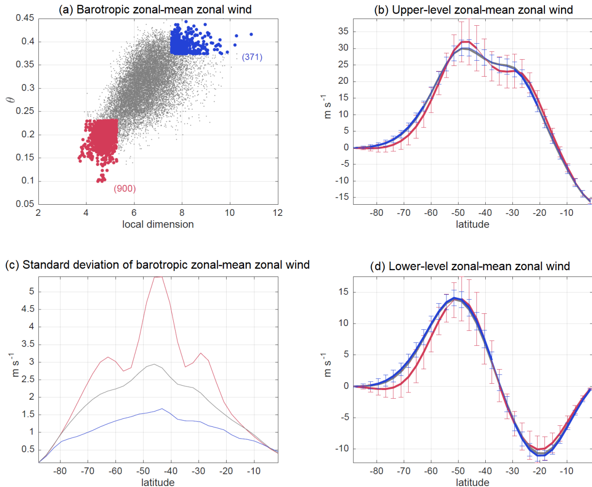
Figure A2. A d - \theta diagram of barotropic zonal-mean zonal wind (a) for simulation no. 2 (see Table A1) and composites over time steps with low ( < 10 th) and high ( > 90 th) percentiles of both d and \theta , upper-level (b) and lower-level (d) zonal-mean zonal wind ( \text{m s}^{-1} ), and (c) barotropic zonal-mean zonal wind standard deviation. The vertical bars in (b) and (d) show the standard deviations of the relevant composites at a given latitude. The red and blue dots (a) and lines and bars (b-d) correspond to low and high d - \theta time steps, respectively, while grey marks all other times (a) or the simulation's climatology (b-d) . The numbers in parentheses in (a) show the sample size of the each composite. Thick lines in (b) and (d) denote latitudes at which the high or low d and \theta composites are significantly different from the simulation's climatology at the 95 % confidence level based on a two-sided Student's t test.
