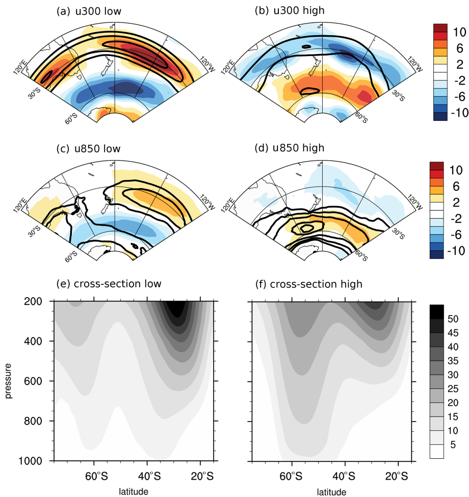
Figure 6. JJA zonal wind composites ( \text{m s}^{-1} ) at 300 hPa ( a, b ) and 850 hPa ( c, d ) as well as zonal-mean zonal wind composite cross sections over the South Pacific domain ( 120^\circ \text{W} – 120^\circ \text{E} ). Separate composites are shown for days displaying low ( a, c, e ) and high ( b, d, f ) values of d and \theta . See text for details. In ( a )–( d ), colours show deviations from the climatology, while contours show absolute values. Contours are every 10 \text{ m s}^{-1} starting from 30 \text{ m s}^{-1} in ( a ) ( b ) and every 3 \text{ m s}^{-1} starting from 6 \text{ m s}^{-1} in ( c, d ).
