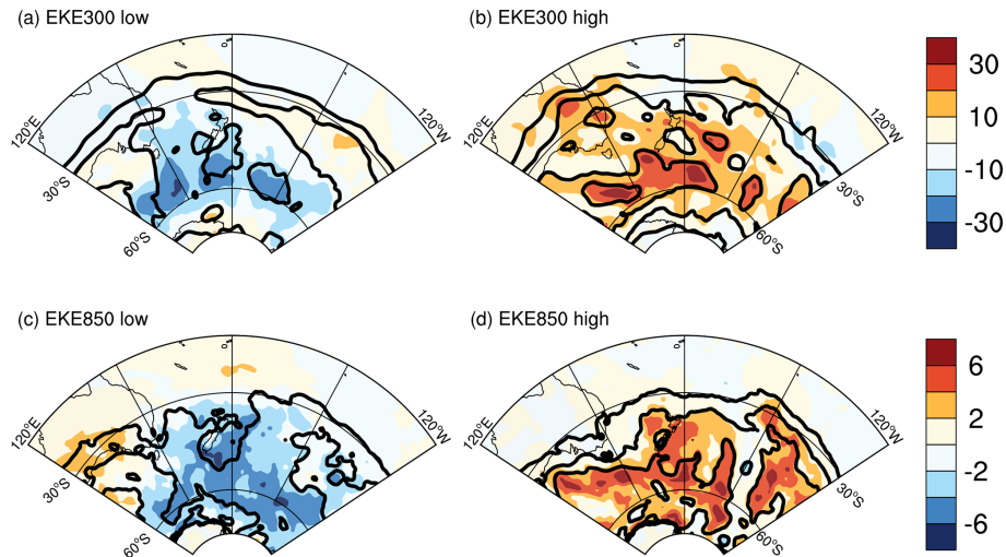
Figure 7. JJA EKE composites ( \text{m}^2 \text{s}^{-2} ) at 300 hPa ( a, b ) and 850 hPa ( c, d ) for days displaying low ( a, c ) and high ( b, d ) values of d and \theta . See text for details. Colours show deviations from the climatology, while contours show absolute values. Contours are every 20 \text{ m}^2 \text{ s}^{-2} starting from 40 \text{ m}^2 \text{ s}^{-2} in ( a, b ) and every 5 \text{ m}^2 \text{ s}^{-2} starting from 10 \text{ m}^2 \text{ s}^{-2} in ( c, d ).
