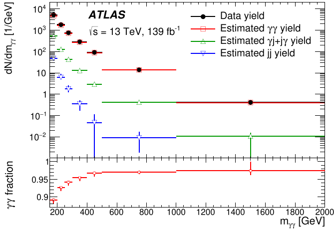
Fig. 1. Diphoton invariant mass distributions of the data after event selection and their decomposition into contributions from genuine diphoton ( \gamma\gamma ), photon+jet ( \gamma j and j\gamma ) and dijet ( jj ) events as determined using the two-dimensional sideband method. The bottom panel shows the sample's purity in diphoton events. Each point in the distributions is plotted in the centre of the corresponding bin. The total uncertainties, including statistical and systematic components added in quadrature, are shown as error bars.
