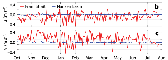
FIGURE 1. (a) Snapshot of current speed averaged over 50–100 m from 1 km numerical simulation of Wang et al. (2020) on December 30, 2008. Note that the 1 km resolution region of the model starts at approximately 75°N in the Nordic Seas. Place names are labeled in white and indicate locations close to the bottom left of each label. Magenta dots mark the locations of the studies shown in Figure 2. For illustrative purposes, two time series of velocity are presented, one representative of very high and one of very low mesoscale variability: (b) eastward velocity [ \text{m s}^{-1} ] and (c) northward velocity [ \text{m s}^{-1} ] at mooring F4 in Fram Strait and mooring Nansen in the Nansen Basin, both marked by red squares in (a). The velocities are averaged over 50–100 m and lowpass filtered with a two-day cutoff. F4, at 78°50'N 7°E in 1,416 m water depth, and Nansen, at 85°18'N 60°E in 3,870 m water depth, have average eddy kinetic energies of 1.3 \times 10^{-2} \text{ m}^2 \text{ s}^{-2} and 6.7 \times 10^{-5} \text{ m}^2 \text{ s}^{-2} , respectively.
