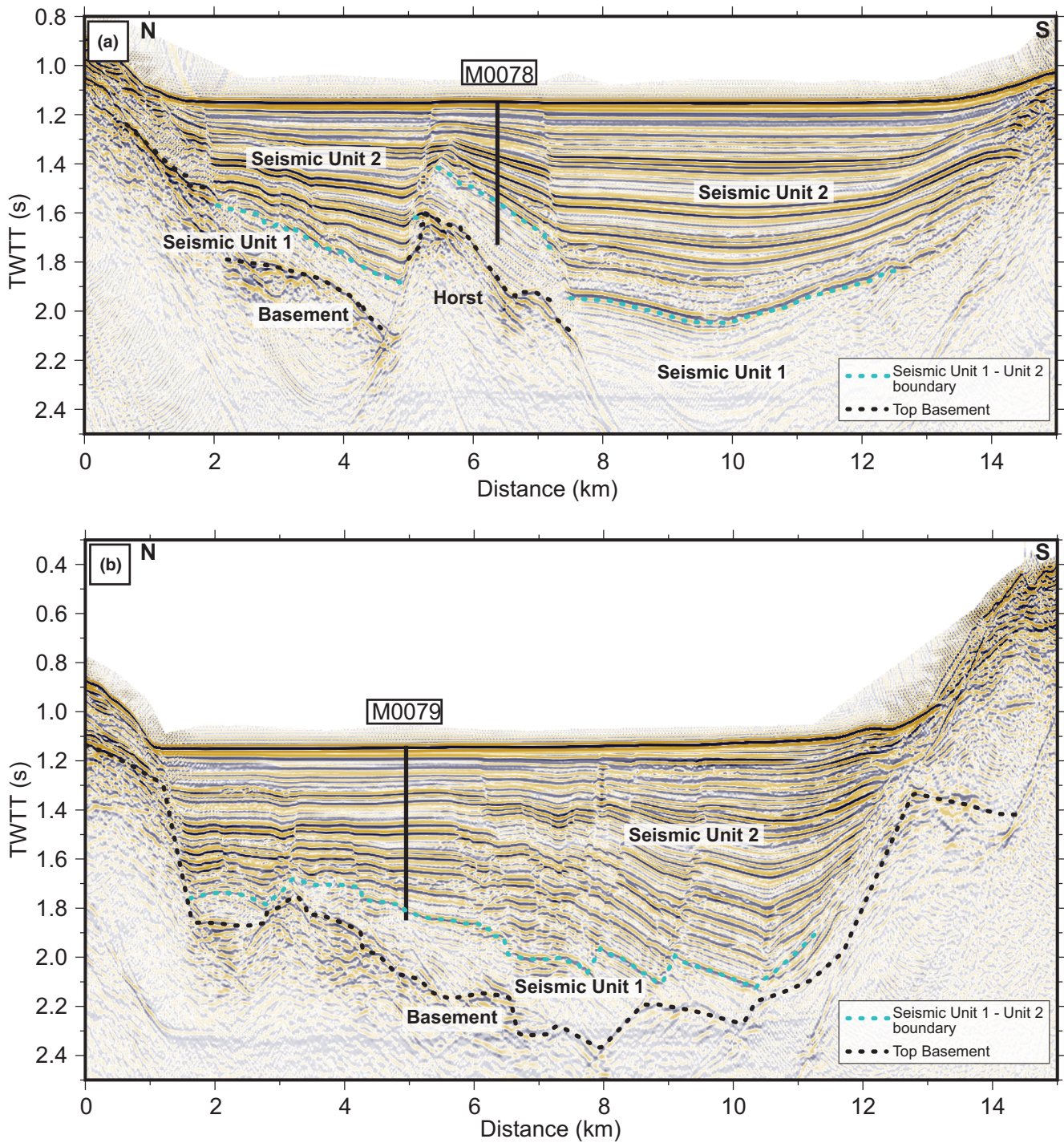
FIGURE 2 Dip section seismic lines crossing through the IODP 381 sites M0078 and M0079. (a) R/V Maurice Ewing line 42, across site M0078, and (b) R/V Maurice Ewing line 41, across site M0079. The black dashed line depicts the top of pre-rift basement and the light blue dashed line depicts the boundary between Seismic Unit 1 and Seismic Unit 2 of Nixon et al. (2016) which are equivalent to IODP Expedition 381 Lithostratigraphic Unit 2 and Lithostratigraphic Unit 1 respectively (McNeill, Shillington, Carter, & Expedition 381 Participants, 2019; Shillington et al., 2019)
