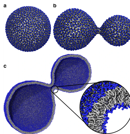
Figure 10: Visualization of vesicle formation from molecular dynamic simulation data [PKWM20]. Reproduced under Creative Commons CC BY license.
