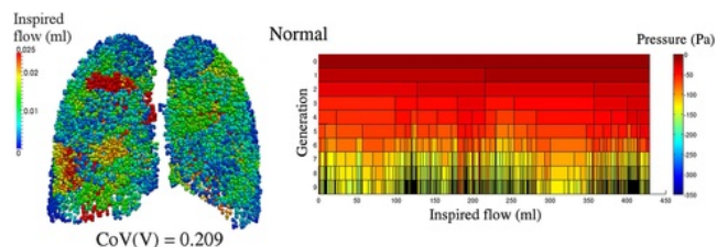
Figure 18: A coupled model of tissue deformation and network airflow that enables predictions of dynamic flow properties [KBV*15]. Reproduced with permission.
