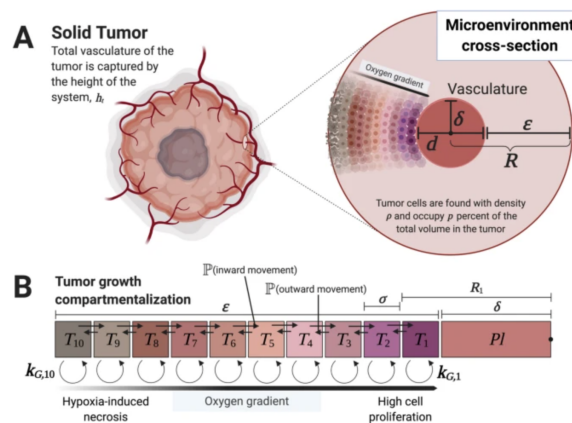
Figure 13: Compartment diagram and parameters for tumor growth [MMF20]. Reproduced under Creative Commons CC BY license.
