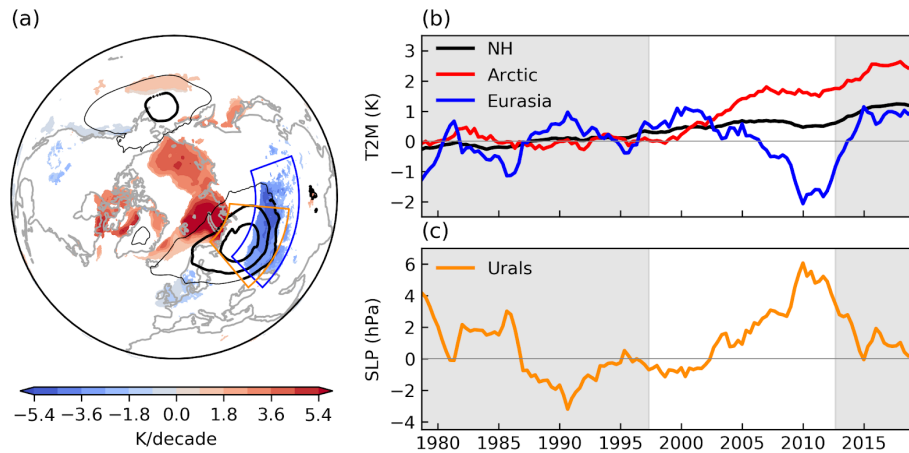
Figure 1. The “warm Arctic–cold Eurasia” pattern and the associated surface circulation. (a) Trends in wintertime 2 m air temperature (shading) and sea level pressure (contours with levels: 3, 6, 9 hPa/decade) in ERA5 reanalysis for 1998 to 2012 over the Northern Hemisphere. Trends for 2 m air temperature are only shown for locations that are significantly different at the 95 % level from the mean Northern Hemisphere trend for the given period. Trends for sea level pressure are shown in thick (thin) contours for locations that are significantly different (not significantly different) at the 95 % level from the mean Northern Hemisphere trend for the given period. The blue (orange) box denotes the Eurasian (Urals) region for calculating the area-averaged indices in panels (b, c) . (b) Indices of area-averaged 2 m air temperature over the Northern Hemisphere (20–90° N, black), Arctic (60–90° N, red), and Eurasia (40–60° N, 45–110° E, blue) from 1979 to 2019. (c) Indices of area-averaged sea level pressure over the Urals (45–70° N, 40–85° E) from 1979 to 2019. (b–c) The indices are constructed from monthly values from December to February. The monthly climatology has been removed relative to a 1979–1998 period and a 5-year running mean applied. The unshaded region corresponds to the period from 1998 to 2012.
