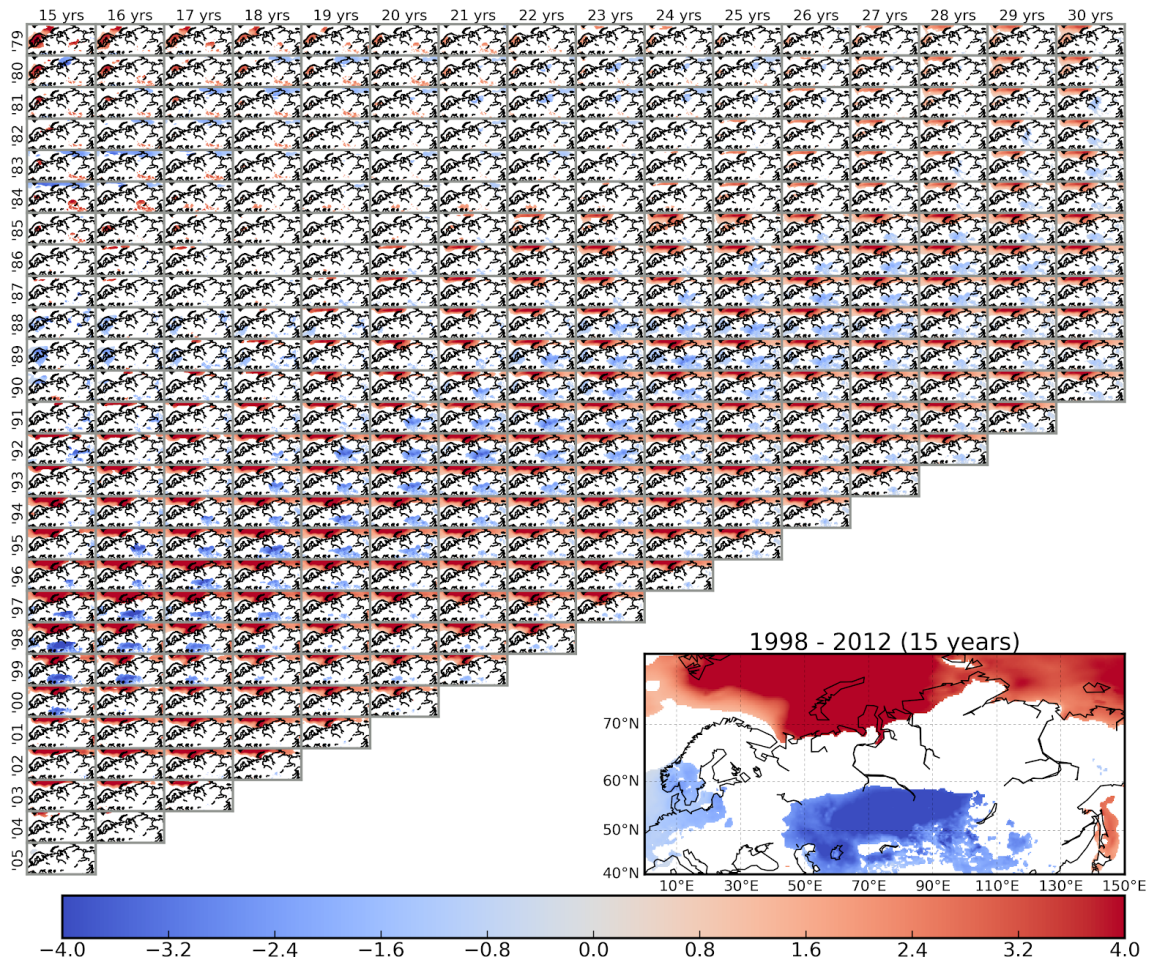
Figure 2. Trends in DJF mean 2 m air temperature in ERA5 reanalysis for periods ranging from 15 to 30 years in length (columns) and for starting years ranging from 1979 to 2005 (rows). The domain shown is 0–150° E and 40–80° N. Trends are only shown when they differ from the Northern Hemisphere trend over the specified period (95 % significance level). The inset (bottom right) shows an expanded view of the panel corresponding to the 15-year period highlighted in Fig. 1a, from DJF 1998 to DJF 2012.
