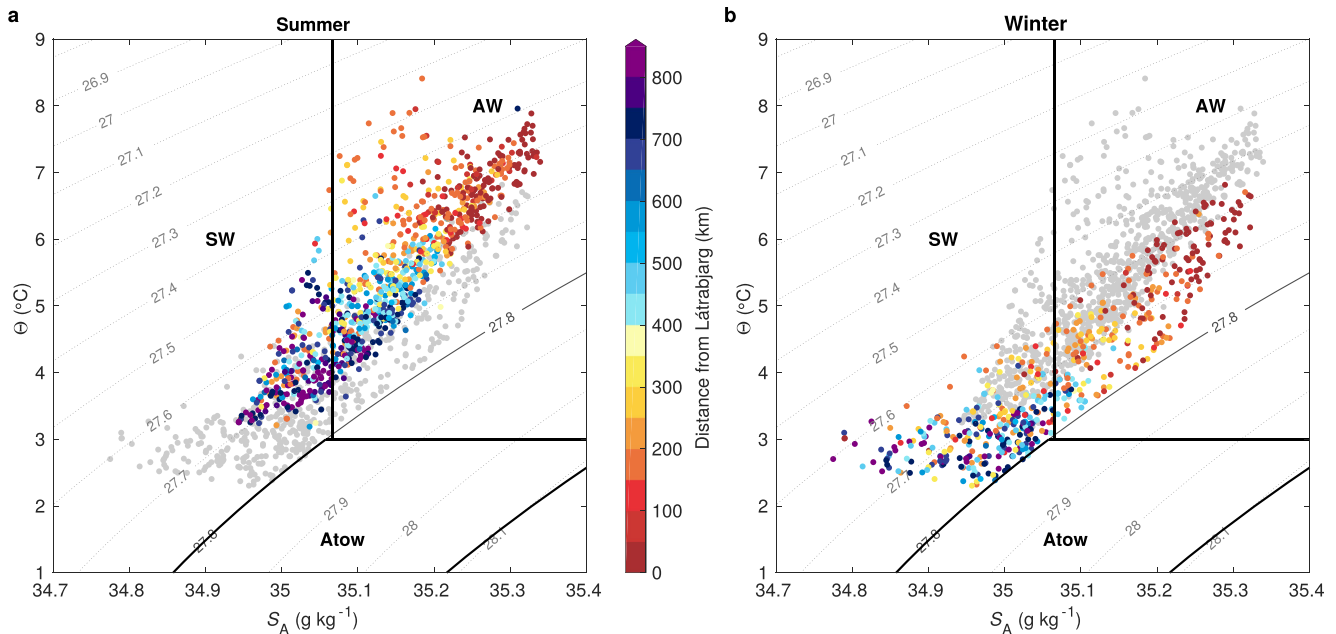
Figure 10. Distribution of hydrographic properties in the North Icelandic Irminger Current (NIIC). \Theta - S_A -diagram of (a) summer and (b) winter hydrographic properties in the NIIC from the historical measurements. The mean of each profile within the core of the NIIC as defined from hydrographic/velocity surveys (see Section 2 for details) is colored by distance from the Látrabjarg transect (Denmark Strait). For reference, the properties of winter and summer are shown by gray dots in the background in panels (a) and (b), respectively. The gray contours are density. The water masses are separated by thick black lines; their acronyms are: AW = Atlantic Water; Atow = Atlantic-origin water; SW = Surface Water.
