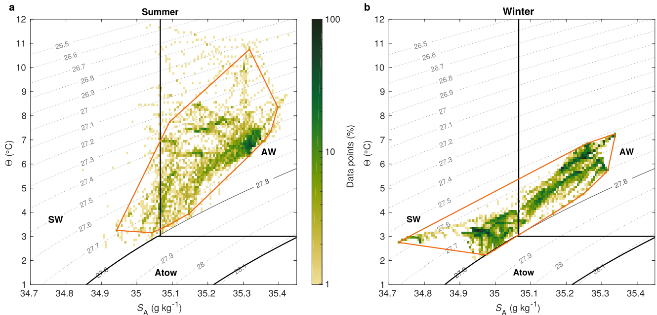
Figure 3. Outline of the North Icelandic Irminger Current (NIIC) core in \Theta - S_A space. Binned (a) summer and (b) winter hydrographic properties from all hydrographic/velocity surveys (see text for details). Note the logarithmic color scale. The core of the NIIC is outlined by the envelope (orange polygon), which encompasses all bins that contain at least 2% of the total number of data points. The gray contours show density. Water masses are separated by thick black lines; their acronyms are: AW = Atlantic Water; Atow = Atlantic-origin water; SW = Surface Water.
