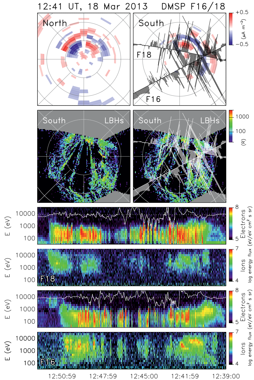
Figure 9. Observations from near-simultaneous passes of the southern hemisphere by Defense Meteorological Satellite Program F16 and F18 around 12:41 UT on 18 March 2013. The auroral observations from the Special Sensor Ultraviolet Spectrographic Instrument on the two spacecraft have been superimposed. At the bottom, electron and ion spectrograms from SSJ/4 on the two spacecraft are shown, with ionospheric flows from the Ion Driftmeter superimposed.
