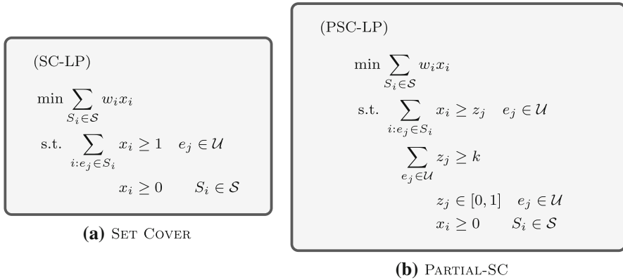
Fig. 1 LP relaxations for covering
