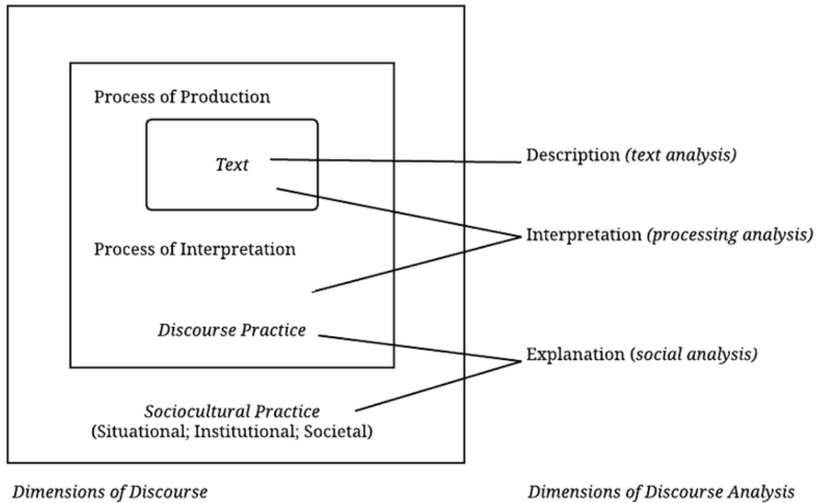
Figur 1: Faircloughs modell for diskursanalyse – Fairclough (2013)
