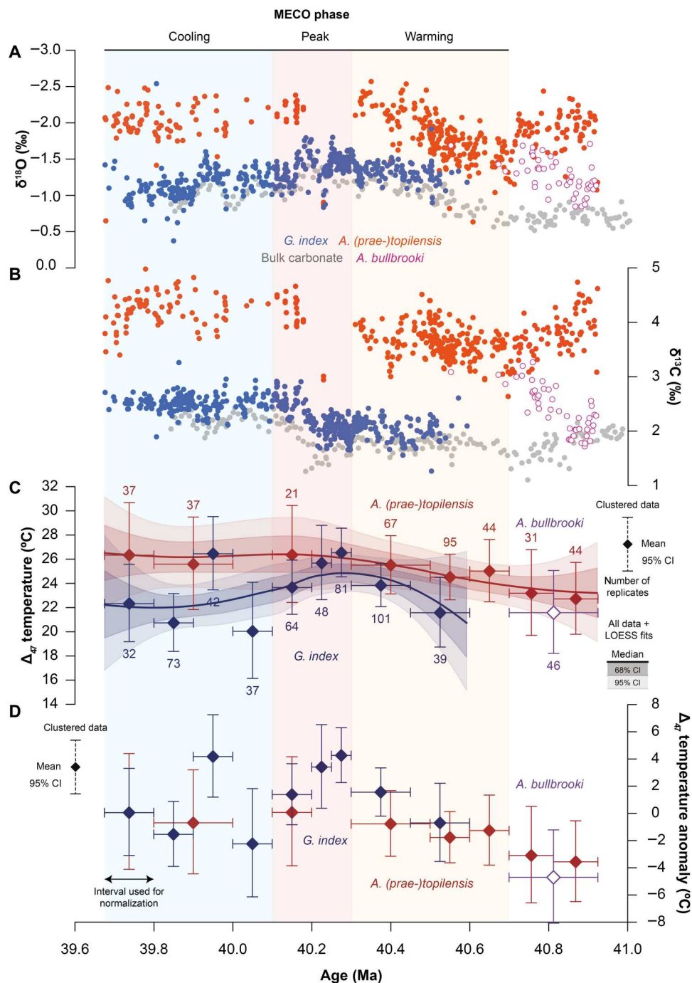
Fig. 2. Foraminiferal stable isotope records and clumped isotope-based temperature records for the MECO interval at Sites U1408 and U1410. (A and B) \delta^{18}O_c and \delta^{13}C_c records for A. (prae-)topilensis (in red), A. bullbrooki (in purple), and G. index (in blue), as well as bulk carbonate (in gray). (C) \Delta_{47} -derived temperatures for A. (prae-)topilensis (in dark red), A. bullbrooki (in dark purple), and G. index (in dark blue). Diamonds represent means of clustered measurements, with vertical error bars indicating 95% confidence intervals (CI), horizontal error bars indicating age ranges of the included measurements, and n representing the number of measurements included (see Materials and Methods). Curves represent the median (thick solid lines), 68% CIs (dark shaded areas), and 95% CIs (light shaded areas) of LOESS fits to all measurements for A. (prae-)topilensis and G. index . (D) \Delta_{47} -derived temperature anomalies for A. (prae-)topilensis (in dark red), A. bullbrooki (in dark purple), and G. index (in dark blue), relative to their respective mean temperatures for the interval between 39.9 and 39.7 Ma. A. bullbrooki was normalized to the A. (prae-)topilensis value. All records are plotted against age following the revised composite age model for U1408 and U1410.
