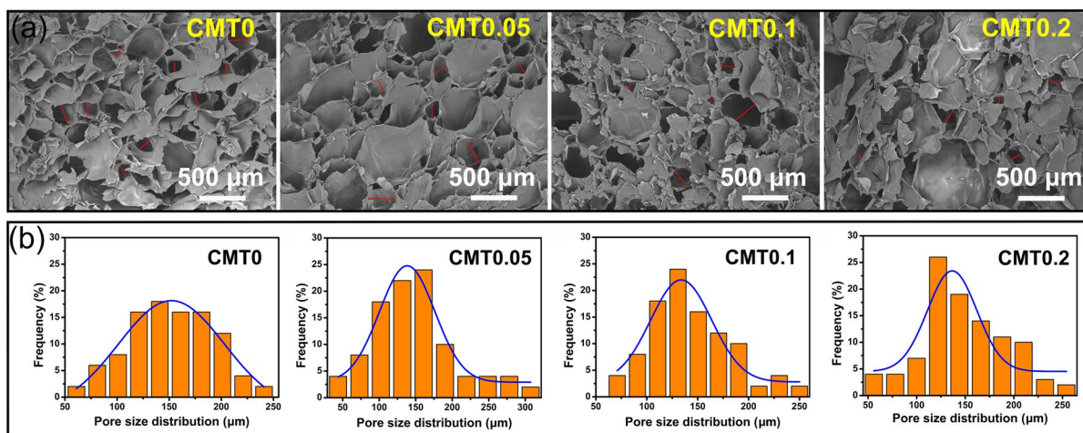
Fig. 3 a The SEM images of CMT; b The pore size distribution of CMT
