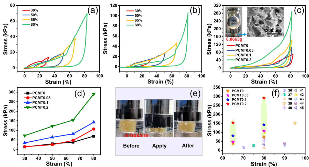
Fig. 8 Stress–strain hysteresis loops of a PCMT0 and b PCMT0.05; c stress–strain hysteresis loops of the PCMT with 80% strain; d Stress–strain hysteresis loops of the PCMT; e
