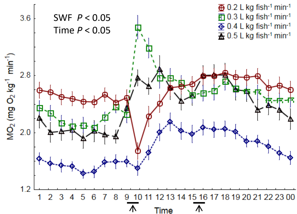
Figure 5. Diurnal specific oxygen consumption ( MO_2 ) in Atlantic salmon post-smolts reared at four different levels of specific water flow (0.2, 0.3, 0.4, and 0.5 L kg fish -1 min -1 ) for 8 weeks. ↑ indicates feeding time. n = 28 days, and all data are given as means \pm SEM.
