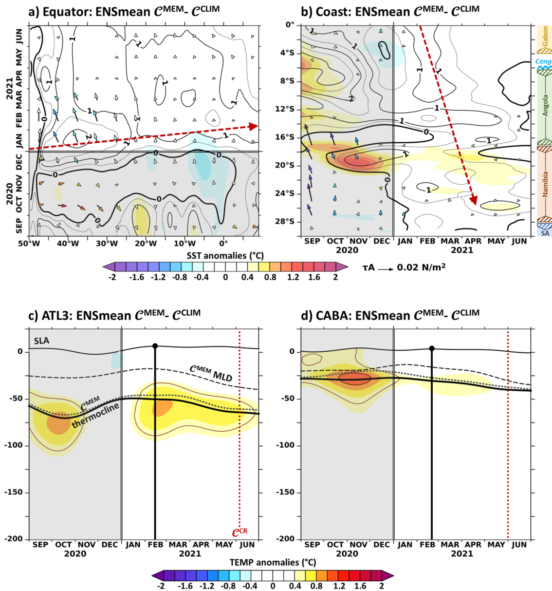
Fig. 6 Coupled response associated with the long-term ocean memory. Same as Fig. 5, but for the ensemble mean of the C^{\text{MEM}} simulations over the period Sep 2020–Jun 2021. The year 2020 has been grayed-out because it consists of the anomalies of the ensemble mean of the \text{CROCO}^{\text{INTER-2020}} forced simulations (relative to \text{CROCO}^{\text{CLIM-2020}} , see Table 1). In the upper panels, red dashed
