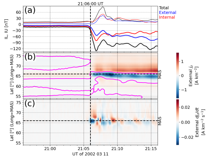
Figure 8. The same as Fig. 2 except for the substorm onset on 11 March 2002 at 21:06:00 UT.
