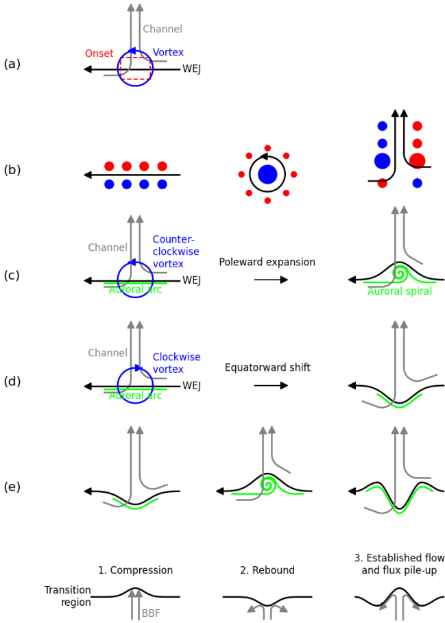
Figure 17. (a) Three basic components of ionospheric equivalent currents observed around substorm onsets: a WEJ, a channel of poleward current with SAPS and DAPS signatures in the eastward and westward current, and a vortex. (b) Curl of the equivalent current density associated with the WEJ, vortex, and channel. The negative curl can be interpreted as an upward FAC and the positive curl as downward FAC under conditions outlined in Sect. 2.4 (c) Superposition of a WEJ and a counterclockwise vortex will produce a poleward bulge in the WEJ. The auroral arc associated with the WEJ is wound into a spiral by the strong upward FAC in the center of the vortex. (d) Superposition of a WEJ and a clockwise vortex will produce an equatorward indentation in the WEJ. The auroral arc associated with the WEJ will be also be shifted equatorward by the strong downward FAC in the center of the vortex. (e) A possible interpretation of the results in terms of magnetospheric processes.
