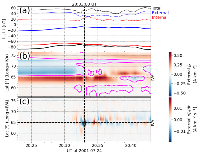
Figure 11. The same as Fig. 2 except for the substorm onset on 24 July 2001 at 20:33:00 UT.
