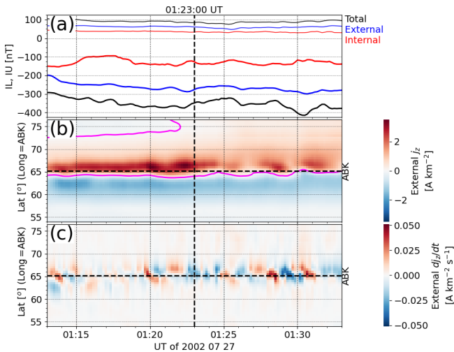
Figure 14. The same as Fig. 2 except for the substorm onset on 27 July 2002 at 01:23:00 UT.
