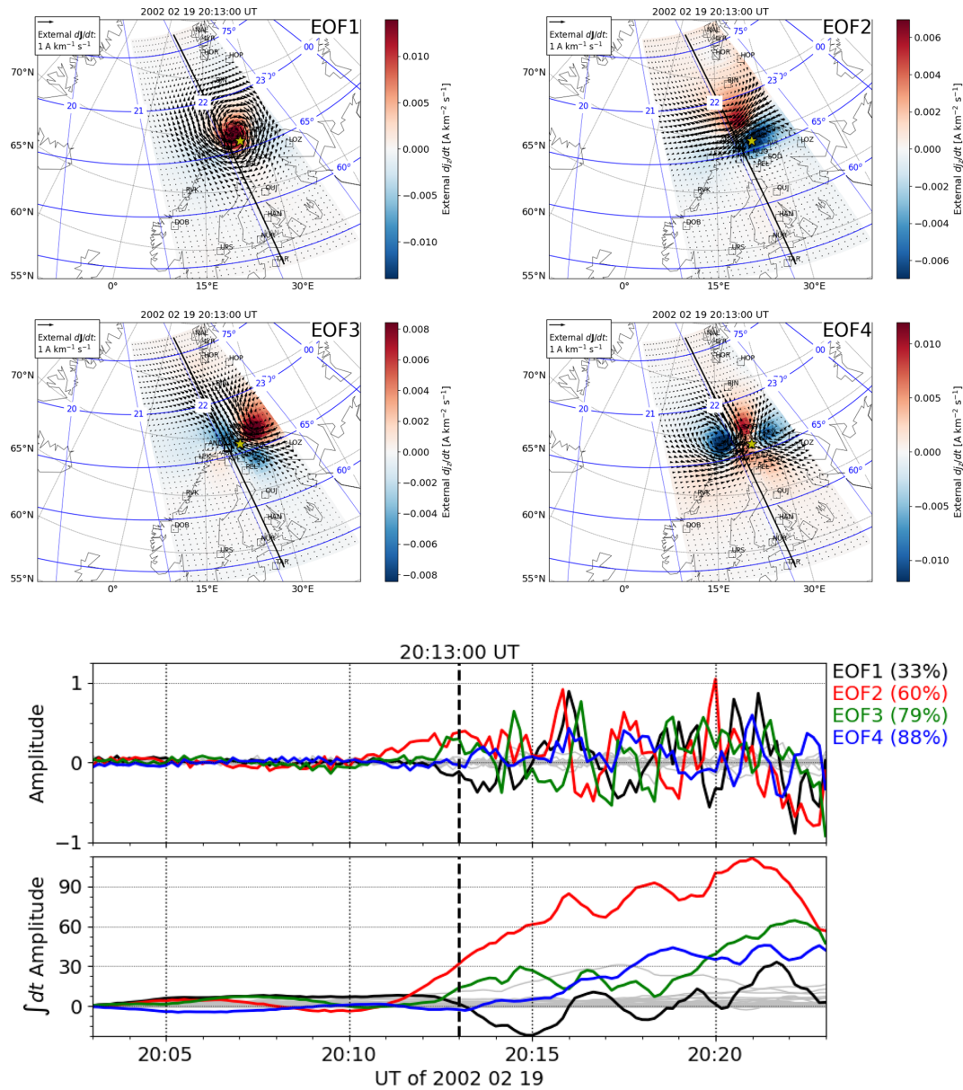
Figure 7. The same as Fig. 4 except for the substorm onset on 19 February 2002 at 20:13:00 UT.
