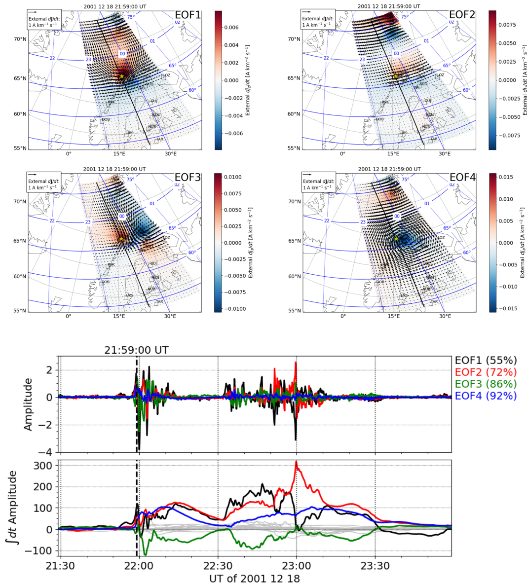
Figure 20. The same as Fig. 4 except for a longer time interval from -30 to +120 min around the substorm onset.
