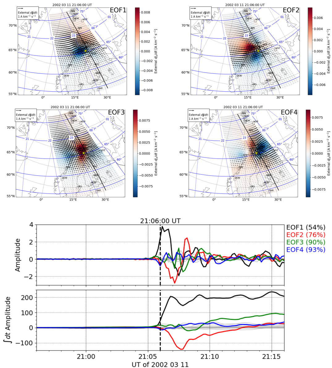
Figure 10. The same as Fig. 4 except for the substorm onset on 11 March 2002 at 21:06:00 UT.
