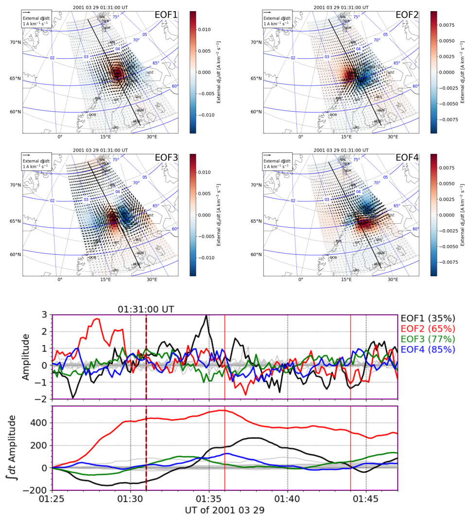
Figure 23. The same as Fig. 4 except for an omega band event on 29 March 2001. The peak times of three omegas are indicated with the red vertical lines.
