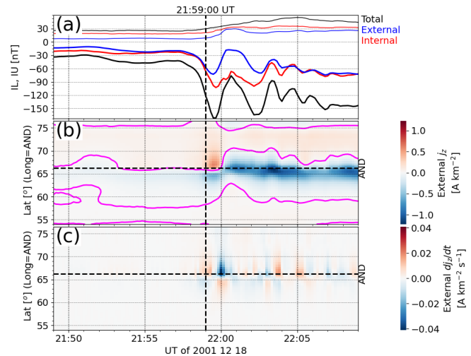
Figure 2. (a) Regional auroral electrojet indices derived from IMAGE data (Kauristie et al., 1996) \pm 10 min around a substorm onset on 18 December 2001 at 21:59:00 UT. The index derived from total (external + internal), external, and internal geomagnetic B_x from all available IMAGE stations is drawn with black, blue, and red color, respectively. The thicker curves show the lower envelope curve of the IL index and the thinner curves show the upper envelope curve of the IU index. The vertical dashed line indicates the substorm onset time. (b) Latitude profiles of external j_z as a function of UT along the longitude of the IMAGE station (AND) located closest to the substorm onset site. The purple curves indicate where j_z changes its sign. (c) Latitude profiles of external 10 \text{ s } dj_z/dt .
