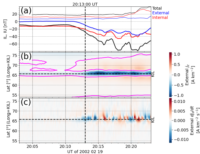
Figure 5. The same as Fig. 2 except for the substorm onset on 19 February 2002 at 20:13:00 UT.
