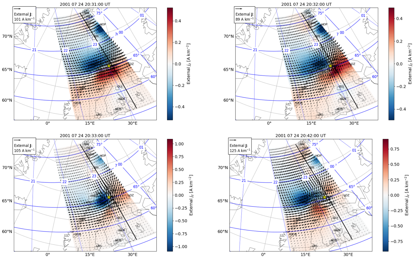
Figure 12. The same as Fig. 3 except for the substorm onset on 24 July 2001 at 20:33:00 UT and without ASC data.
