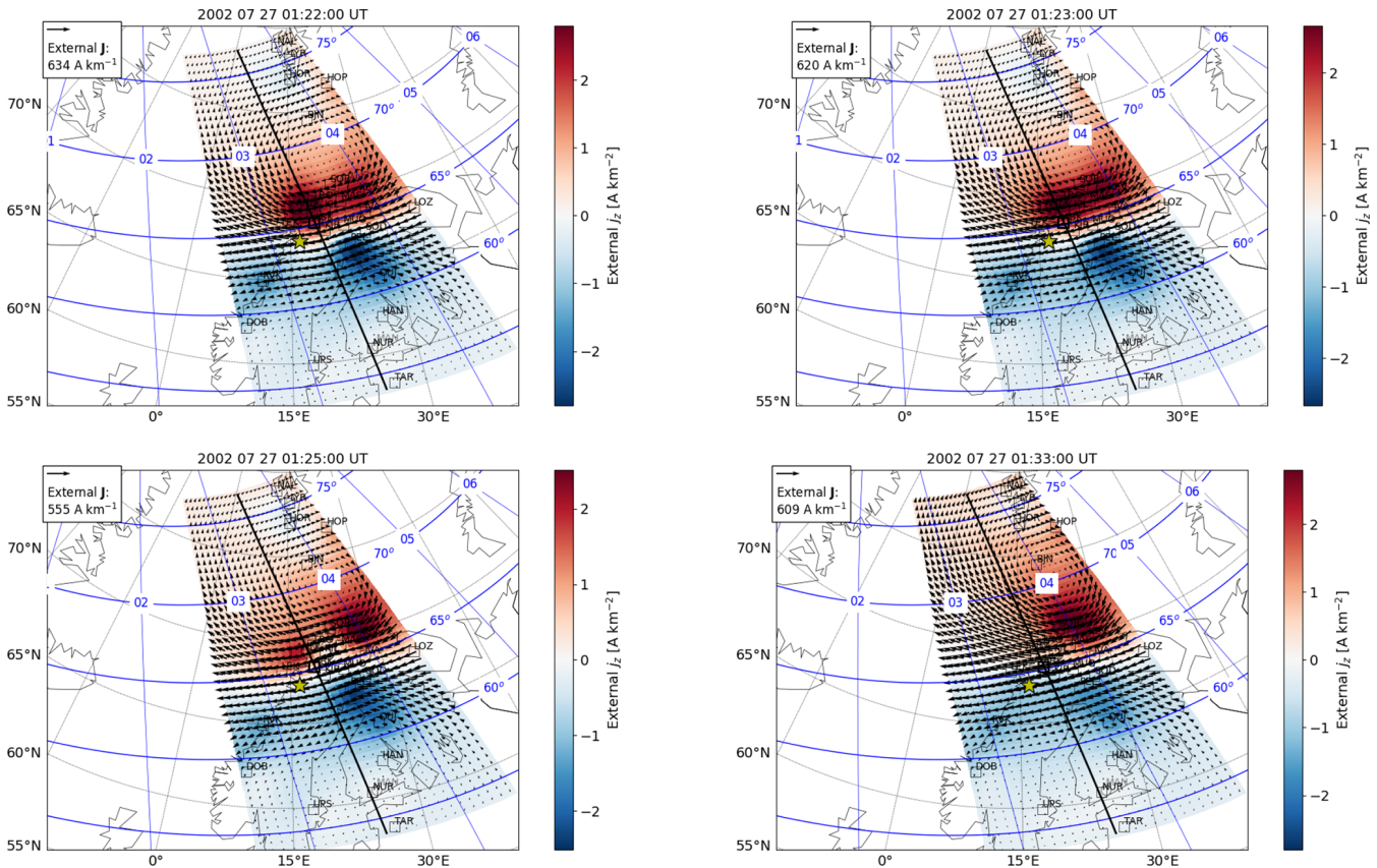
Figure 15. The same as Fig. 3 except for the substorm onset on 27 July 2002 at 01:23:00 UT and without the ASC data.
