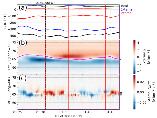
Figure 21. The same as Fig. 2 except for an omega band event on 29 March 2001. The peak times of three omegas (01:31:00, 01:36:00, and 01:44:00 UT) are indicated with the red vertical lines.
