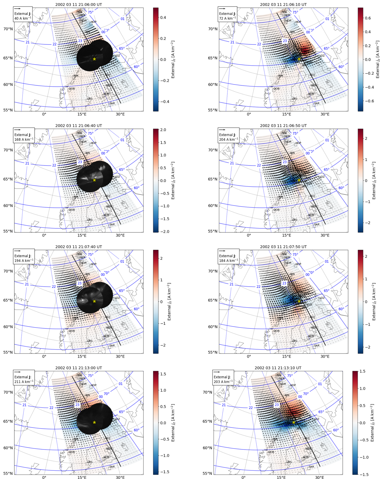
Figure 9. The same as Fig. 3 except for the substorm onset on 11 March 2002 at 21:06:00 UT. The ASC images have been mapped to 120 km altitude.
