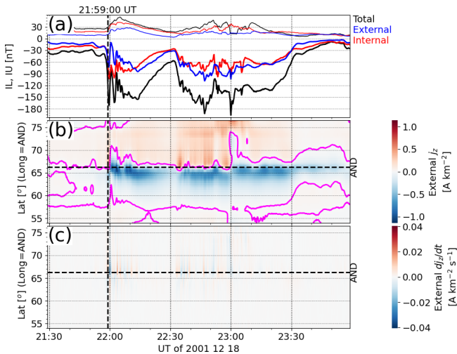
Figure 19. The same as Fig. 2 except for a longer time interval from -30 to +120 min around the substorm onset.
