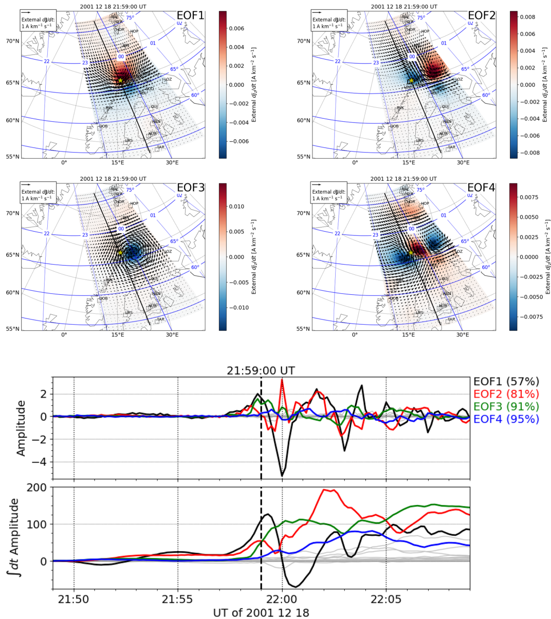
Figure 4. Four most significant empirical orthogonal functions (EOF1–EOF4) or spatial modes of dJ/dt and dj_z/dt , their amplitudes or temporal modes, and time integrals of the amplitudes for \pm 10 min around a substorm onset on 18 December 2001 at 21:59:00 UT. The cumulative percentage of the variance explained by each EOF is indicated in the parentheses. The grey curves (117 curves) correspond to the rest of the EOFs having a smaller contribution.
