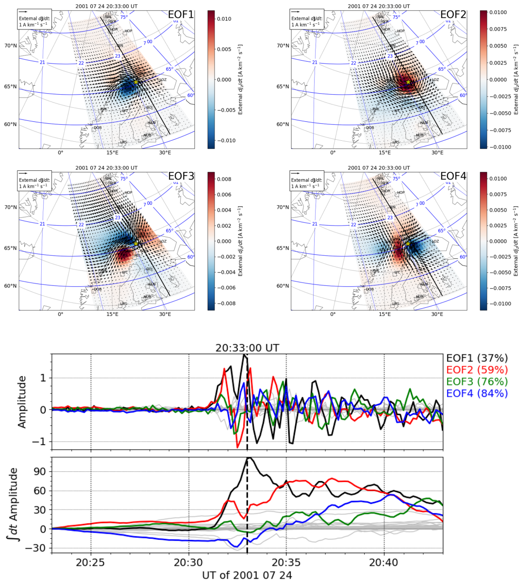
Figure 13. The same as Fig. 4 except for the substorm onset on 24 July 2001 at 20:33:00 UT.
