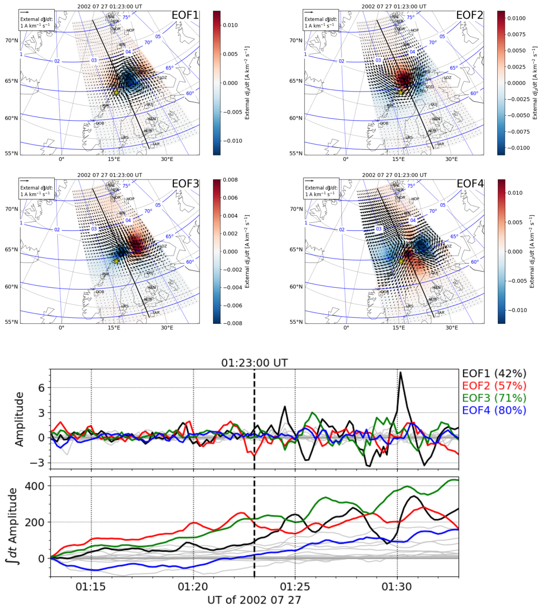
Figure 16. The same as Fig. 4 except for the substorm onset on 27 July 2002 at 01:23:00 UT.
