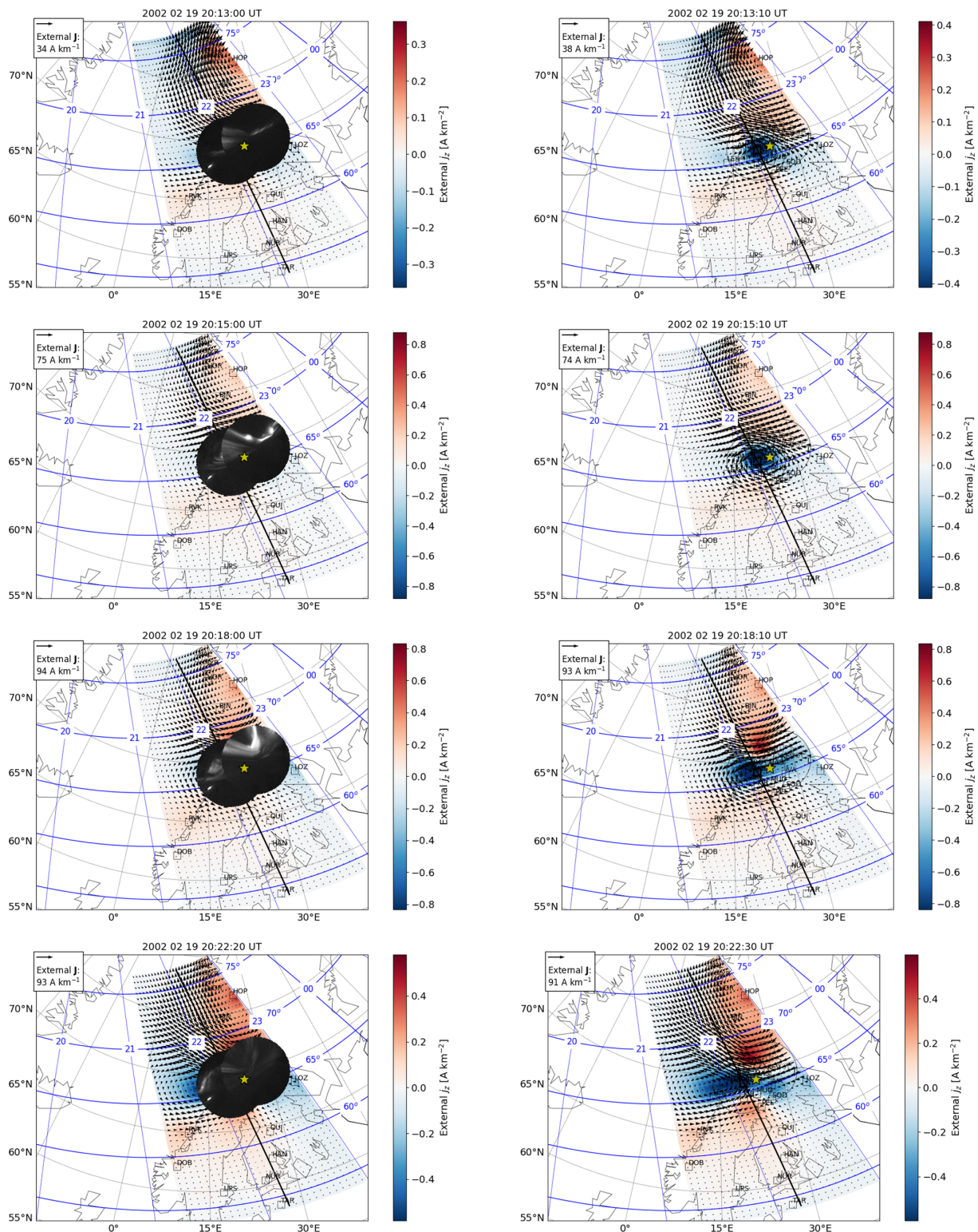
Figure 6. The same as Fig. 3 except for the substorm onset on 19 February 2002 at 20:13:00 UT. The ASC images have been mapped to 120 km altitude.
