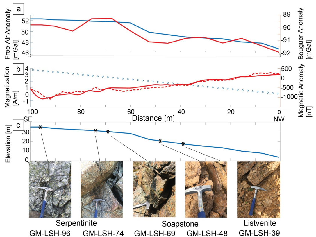
Figure 2. Summary of the field survey along the 100 m transect at Monarch Mountain, Atlin. (a) Crustal scale gravity (top: free air (blue) Bouguer (red) anomalies, with 2.67 \text{ g/cm}^3 reduction density (See Text S1 in Supporting Information S1).) and (b) magnetic anomaly measurements (observed (red dotted; nT) and forward model results (red solid; nT) based on magnetization model (blue circles, \text{Am}^2 )). (c) Changes in elevation over the survey transect. All measurements were taken with a 1 m sampling interval. The stars indicate the locations of the five representative rock samples shown in the imagery.
