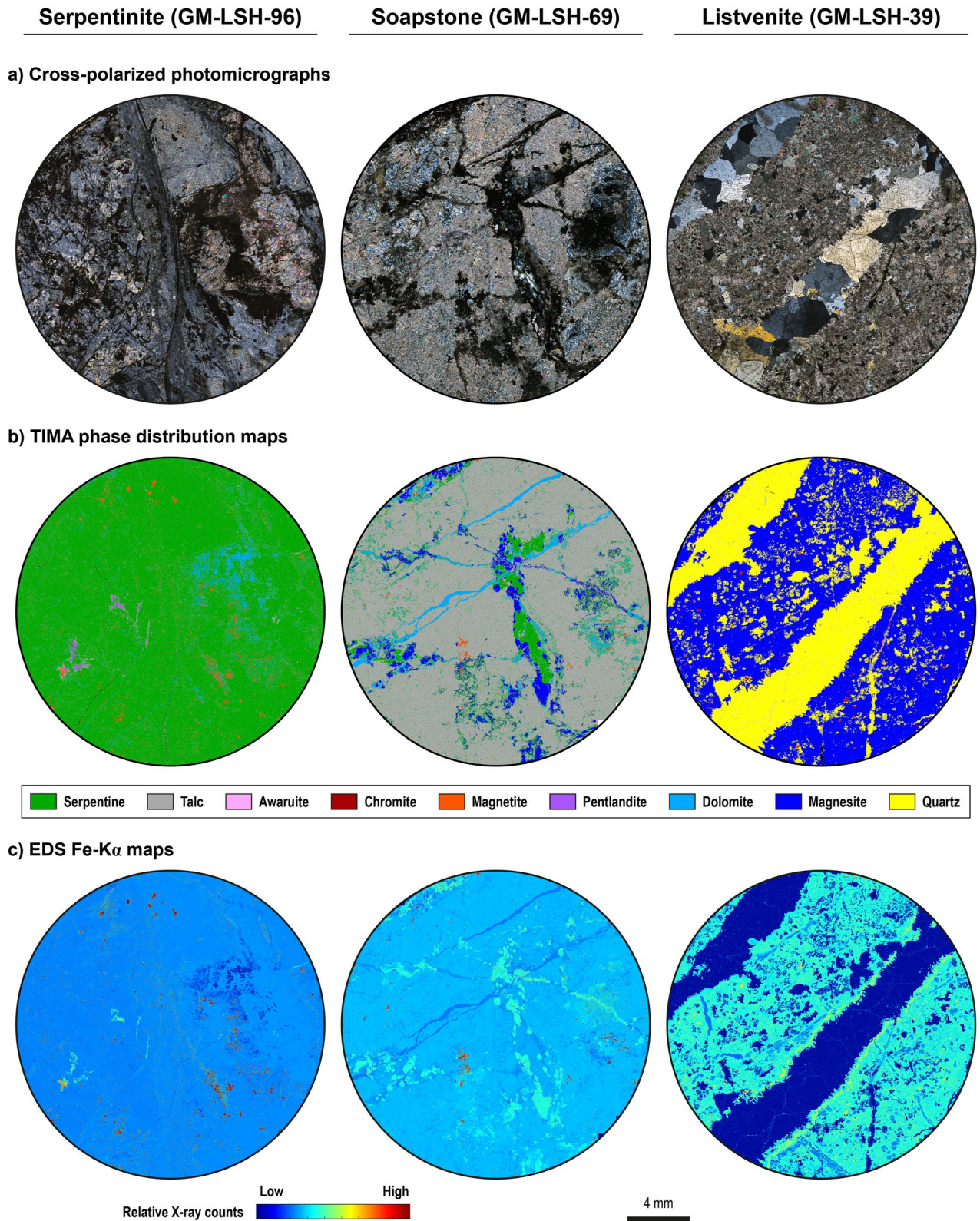
Figure 3. Microtextural observations in representative samples of the serpentinite, soapstone transition zone, and listvenite. (a) Cross-polarized full thin section photomicrographs. (b) energy dispersive spectroscopy phase maps. (c) Fe K \alpha element distribution maps. Note in (c) the Fe enrichment in nonoxide matrix minerals from the serpentinite to the listvenite.
