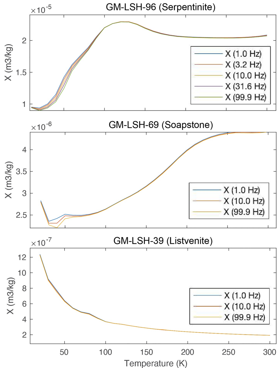
Figure 5. Frequency-dependent susceptibility measurements of three representative lithologies: serpentinite (GM-LSH-96), soapstone (GM-LSH-69), and listvenite (GM-LSH-39).
