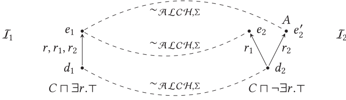
Fig. 5. Interpretations \mathcal{I}_1 and \mathcal{I}_2 illustrating Example 5.9.
