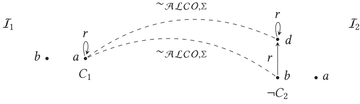
Fig. 4. Interpretations \mathcal{I}_1 and \mathcal{I}_2 illustrating Example 5.7.
