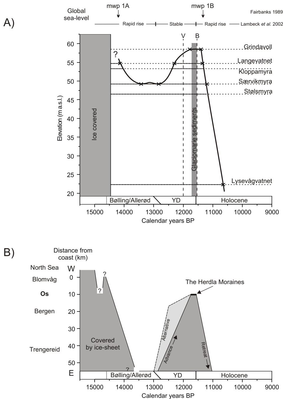
Figure 11 (A) The relative sea-level curve for the Os area based on the calendar year ages of isolation and ingression contacts in the studied basins (Table 3). The stratigraphy in each basin is plotted as a full line for periods with marine sedimentation and a dotted line for periods of lacustrine sedimentation. The Vedde Ash (V) and the pollen-stratigraphical Betula rise (B) are plotted as dashed vertical lines. The timing of the YD glacier maximum in this area (Bondevik and Mangerud, 2002) defined by glaciomarine sediments in basins, is shown as a shaded bar. The course of the global glacio-eustatic sea-levels (Fairbanks, 1989; Lambeck et al. , 2002) are indicated above the sea-level curve. Sea-level data from Kløppamyra and Stølsmyra (Fig. 1) are also included (Bondevik and Mangerud, 2002). (B) Time–distance diagram of ice-front variations in the Bergen district plotted on a similar and vertically aligned time-scale, modified from Mangerud (1977). An alternative course of the YD glacier advance, outlined from the sea-level curve from Os (above), is included
