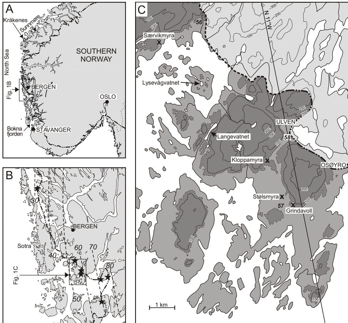
Figure 1 The area studied is located in Os about 25 km south of Bergen on the western coast of Norway. (A) Key map of southern Norway, with YD ice margin (dot-dash lines) (Mangerud, 2004). (B) The YD isobases (dashed lines) are constructed from marine limit terraces (*) deposited in front of the YD ice-marginal Herdla Moraines (dot-dash lines) (Aarseth and Mangerud, 1974). (C) Location of the sites investigated, with the elevation (m a.s.l.) of marine limit terraces (numbers in italic) and the baseline for the shoreline displacement curve (58 m Younger Dryas isobase). Dark grey fill indicates areas above the marine limit, grey indicates present land below the marine limit and light grey shows areas within the former YD ice-sheet. Dot-dash line indicates ice-sheet margin from Aarseth and Mangerud (1974); short-dash line indicates ice-sheet margin based on other criteria
