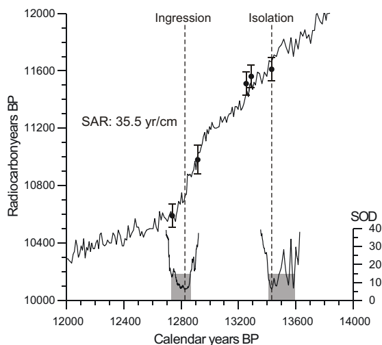
Figure 10 Five of the 14 C dates from Særvikmyra wiggle matched to the Cariaco Basin calibration curve (Hughen et al. , 2000). The lowest sum of differences (SOD) was obtained with a sediment accumulation rate (SAR) of 35.5 yr cm -1 , and positioning the depth of the isolation contact at 13 430 cal. yr BP and the ingressions contact at 12 830 cal. yr BP. Shaded grey areas show age intervals with SOD < 15, which are regarded as a good fit (Table 3). Radiocarbon dates are plotted at ±2σ according to the best fit from the wiggle matching. For further explanation see text
