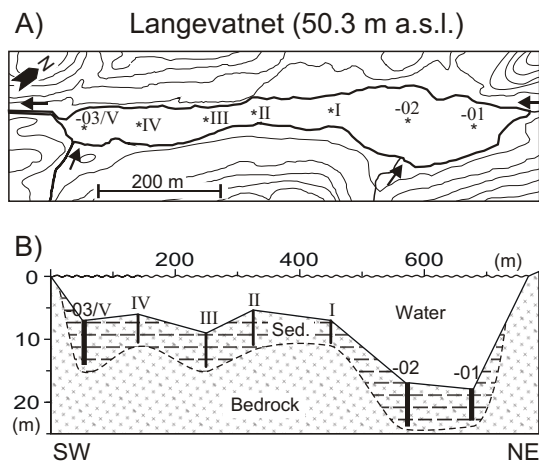
Figure 4 (A) Map of Langevatnet (note the oblique arrow towards north). Cores marked in Roman numerals are Russian peat cores, whereas arabic numbers mark the 110 mm piston cores (01 = 505-01, 02 = 505-02, 03 = 505-03). Contour interval of 10 m. Three minor creeks and the outlet of the lake are marked by arrows in flow direction. (B) Longitudinal profile. Vertical scale is in metres below the lake surface (50.3 m a.s.l.) and horizontal scale in metres from the outlet sill
