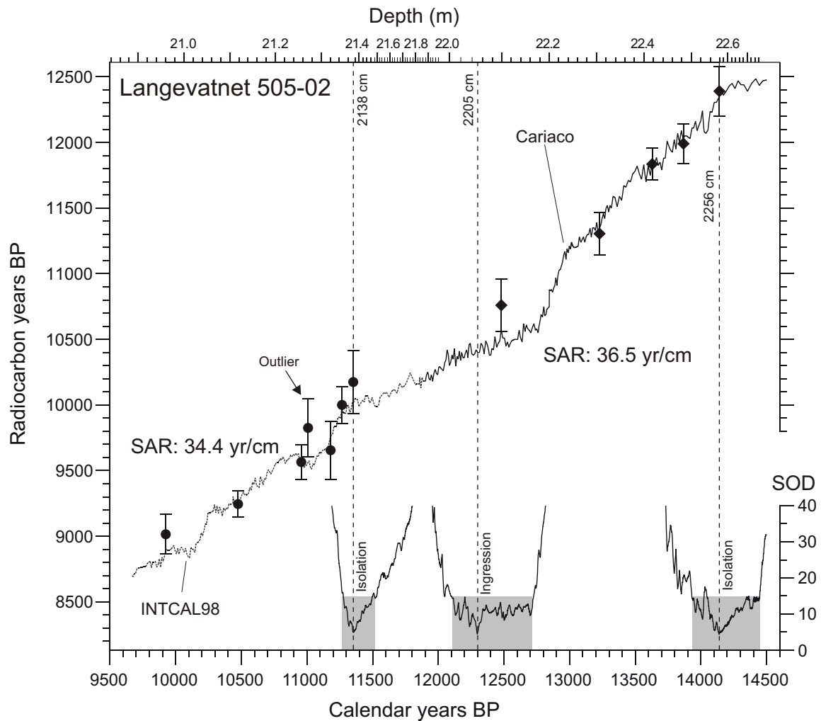
Figure 8 The 14 C dates from the lacustrine unit younger than 10 200 14 C yr BP were wiggle matched to the INTCAL98 calibration curve (Stuiver et al. , 1998). The best fit, i.e. the lowest sum of differences (SOD), was obtained with a constant sedimentation rate of 34.4 yr cm -1 and with an age of the isolation contact (2138 cm) of 11 350 cal. yr BP. The outlier date TUa-2178 (Table 1) was not used. The 14 C dates below the Vedde Ash Bed were wiggle matched to the Cariaco basin data (Hughen et al. , 2000). Best fit was obtained with a constant sedimentation rate of 36.5 yr cm -1 and a location of the isolation contact (2256 cm) at 14 140 cal. yr BP and the ingress ion contact (2205 cm) at 12 300 cal. yr BP. Radiocarbon dates are plotted with ± 2σ according to the best fit from the wiggle matching. Shaded grey areas show age interval with SOD < 15, which are regarded as a good fit (Table 3). Non-linear depth scale is according to the age model shown in Fig. 9. For further explanation see text
