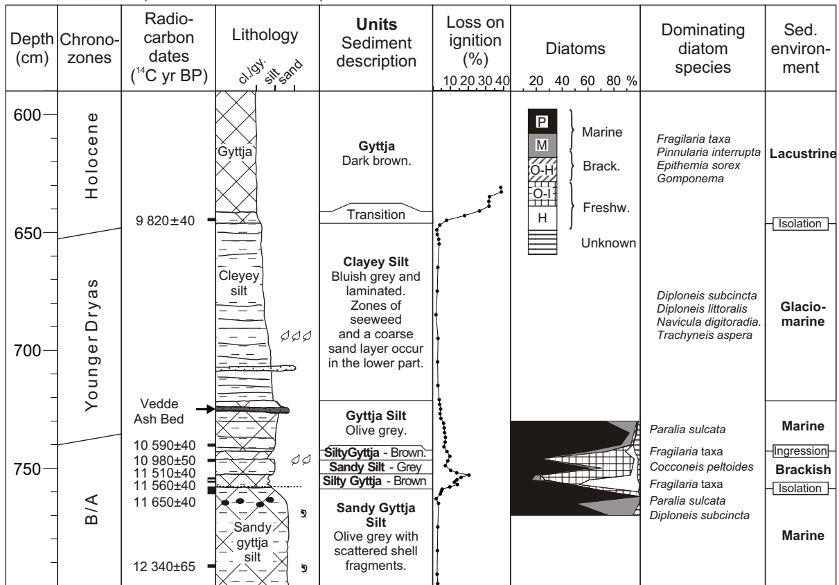
Figure 6 The stratigraphy of Særvikmyra (core 02-151/152). Diatom analysis is conducted for the interval 770–730 cm; other diatom information is based on only a brief microscopic check of slides. Diatom salinity groups: P, polyhalobous; M, mesohalobous; O-H, oligohalobous halophilous; O-I, oligohalobous indifferent; H, halophobous. See Table 2 for details about dates. Detailed diatom diagram from Særvikmyra is shown in Appendix 4
