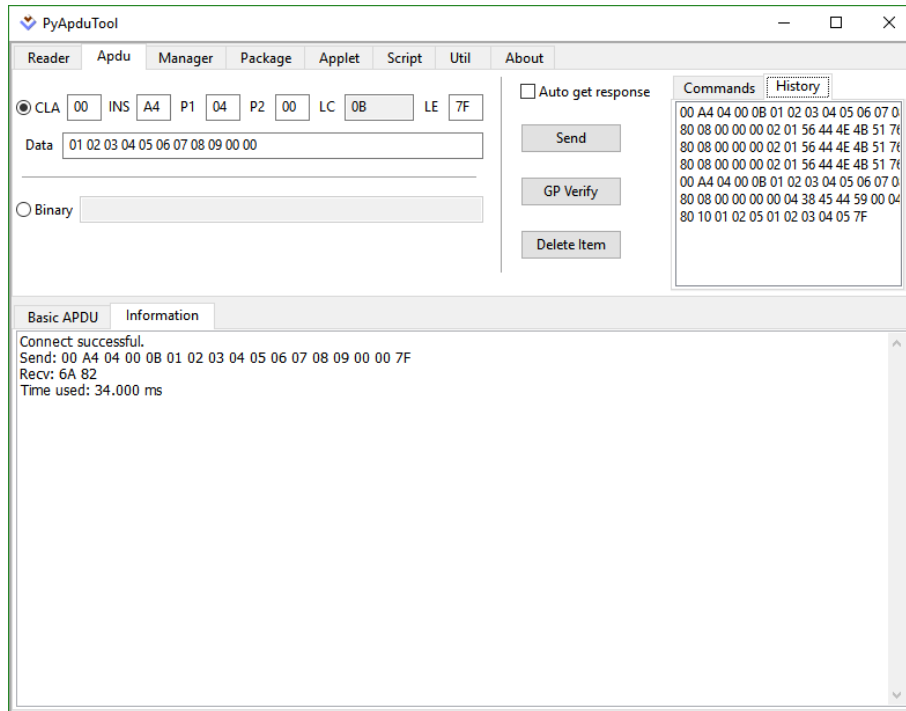
Figure 3.3: Select APDU sent to smart card via PyApuTool
