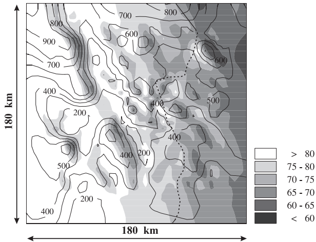
Figure 5: As Figure 4a, but for 4.5 (Nest 2 in Figure 1) kilometres grid distance.
