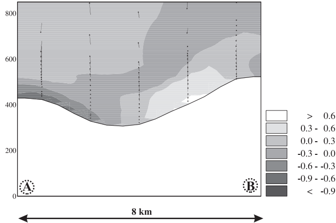
Figure 10: Vertical cross-section showing the temperature difference between the modified and the reference run at 09 UTC 21 September. The arrows indicates the vertical velocity in the cross-section, ranging from -1 to +1 \text{ m s}^{-1} The cross-section is indicated on Figure 9b.
