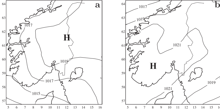
Figure 3: (a) Mean SLP at southern part of Norway 12 UTC 20 September 1994. (b) as figure (a), but at 12 UTC 21 Sept. Ticks at axes are latitude and longitude.
