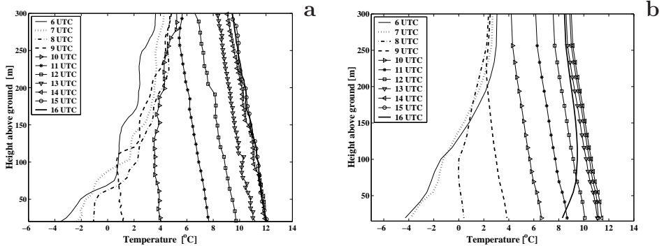
Figure 6: (a) Observed temperature soundings 21 September 1994 in the observation point marked at Figure 2. (b) Modelled sounding in the reference run.
