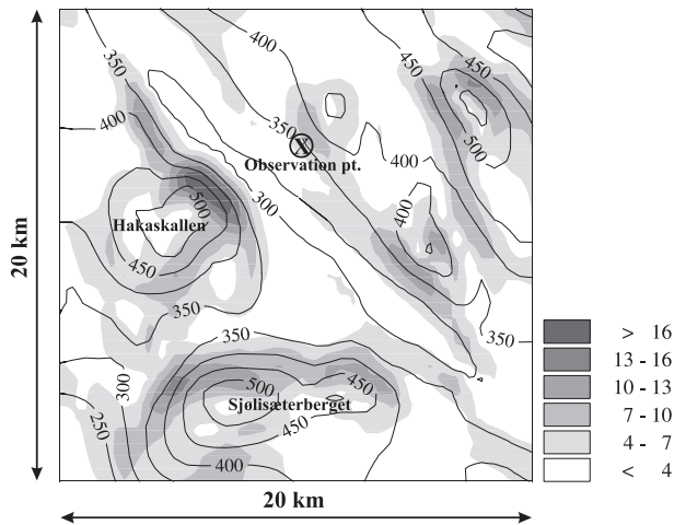
Figure 2: Shading: slope angles (degrees), lines: topography for Finnsko-gen, Nest 4. The x-mark indicates the observation site.
