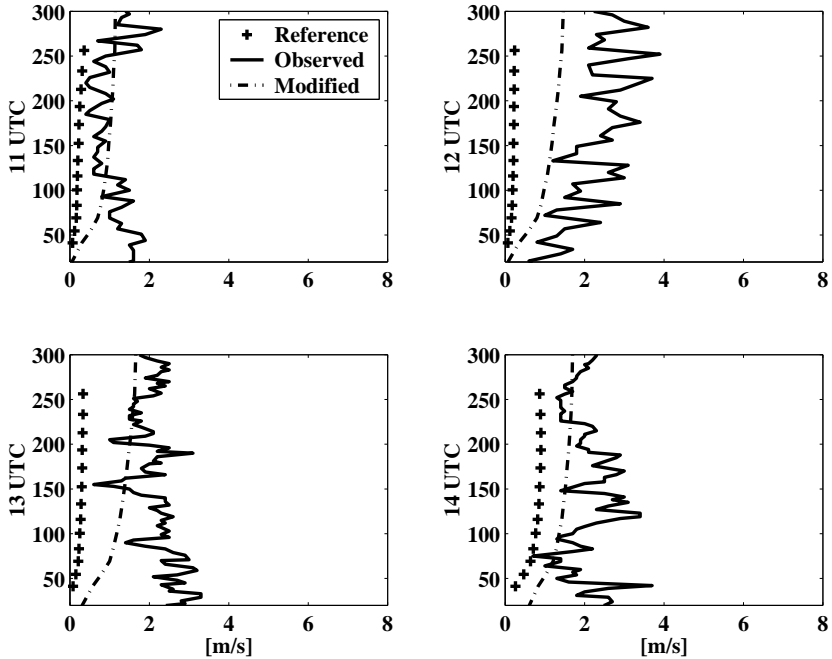
Figure 11: Observed and modelled profiles of wind speed ( \text{ms}^{-1} ) at the site marked on Fig 2.
