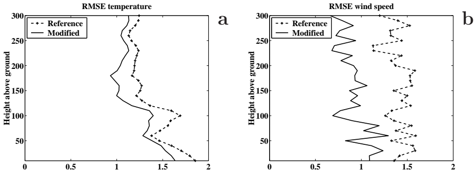
Figure 12: (a) RMSE in temperature between 06 UTC and 16 UTC 21 September. (b) RMSE in wind speed.
