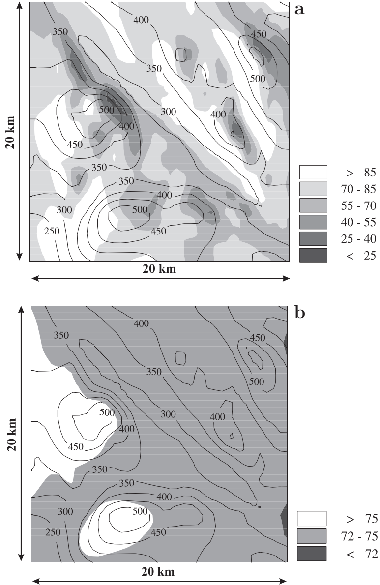
Figure 4: (a) Calculated net shortwave radiation (SW) at the surface, Wm^{-2} , in the modified-run at 16 UTC 20, September 1994. Shaded areas show minima of SW, white areas maximum. Isolines are height of topography. The model grid distance is 500 meters. (b) The reference run.
