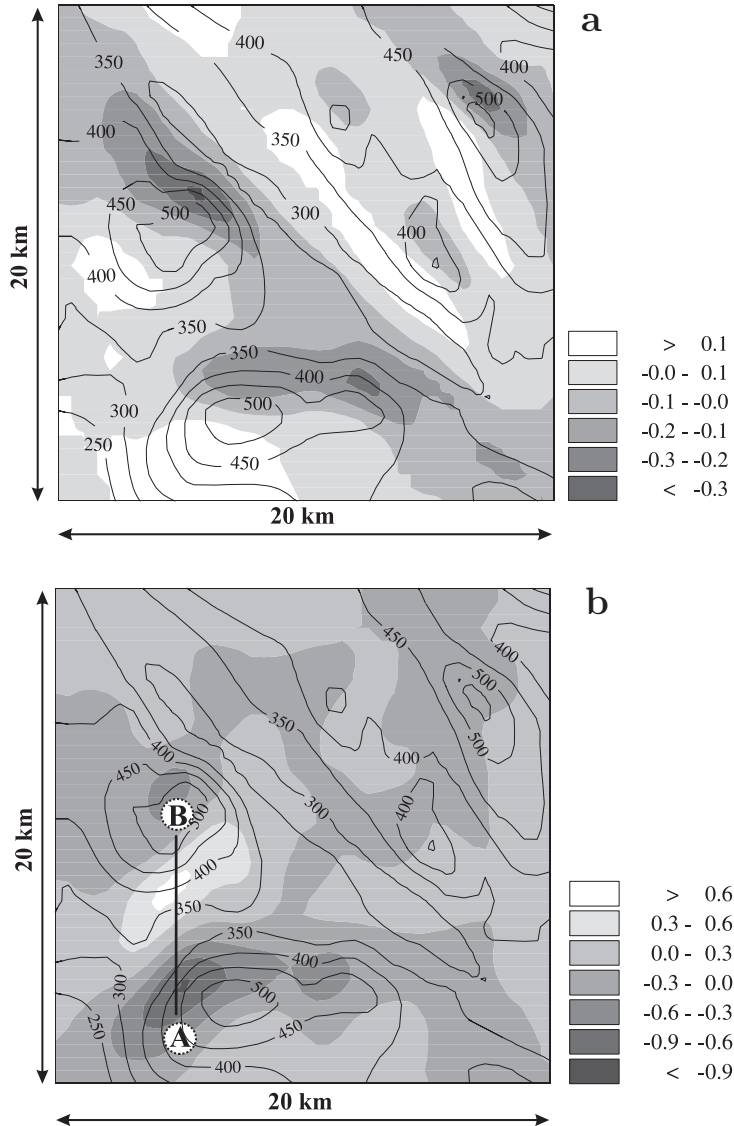
Figure 9: (a) Difference in temperature at the lowest model layer (20 meter) between the modified run and the reference run at 13 UTC 20 September 1994 ( T_{\text{modified}} - T_{\text{reference}} ). (b) As (a), but at 09 UTC 21.09. The marked line and with A – B indicates the vertical cross-section shown on Figure 10.
