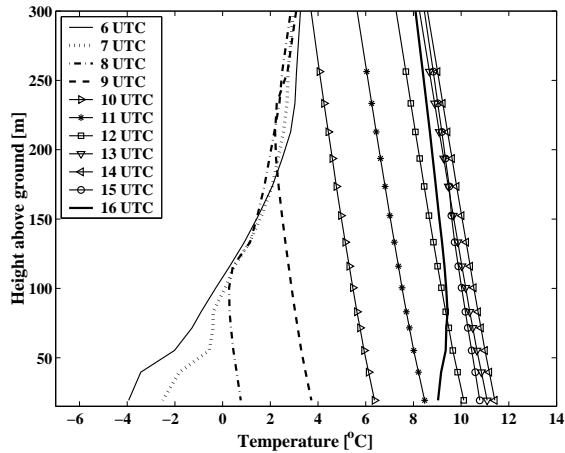
Figure 8: Modelled temperature soundings in the modified run .
