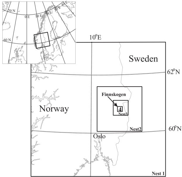
Figure 1: Nesting of MM5 domains. All domains are 40 \times 40 grid points with the resolution 13.5\text{km} \leftrightarrow 4.5\text{km} \leftrightarrow 1.5\text{km} \leftrightarrow 0.5\text{km} (Nest1...Nest4). The upper left figure shows the position of Nest 1 on an European scale.
