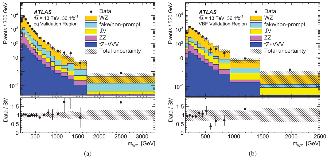
Fig. 3. Observed and expected distributions of the WZ invariant mass in (a) the q\bar{q} validation region and (b) the VBF validation region. The points correspond to the data and the histograms to the expectations for the different SM processes. The uncertainty in the total background prediction, shown as bands, combines statistical, theory and systematic contributions. The bin sizes were chosen to reflect the resolution of a reconstructed signal, and the width of the previous to last bin is used to scale the bin contents. The last bin contains the overflow.
