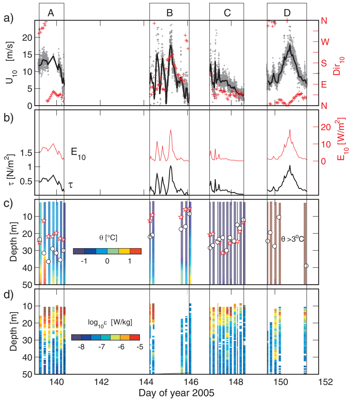
Figure 3. Overview of along-track a) wind speed, U_{10} , and direction b) wind stress, \tau and work, E_{10} and MSS derived set-averaged color-coded profiles of c) potential temperature, \theta and d) dissipation, \varepsilon . Wind data are recorded at \sim 10\text{m} from the ship weather station. The 1-min wind velocity record (speed shown as gray crosses in a) are hourly vector-averaged (black trace in a), interpolated for missing data prior to calculation of direction, stress and wind work. Time series cover varying geographic locations (Fig. 1). The duration of occupation of stations is bounded by vertical lines with stations names indicated at top. Station D is in open water with temperature > 3^\circ\text{C} in the upper 50m. In c) circles are the mixing layer depth whereas red stars are the mixed layer depth. Typical duration of each MSS set is about 1-h, however the width of the color-coded columns in c) and d) are arbitrary, \sim 3\text{h} , for clarity.
