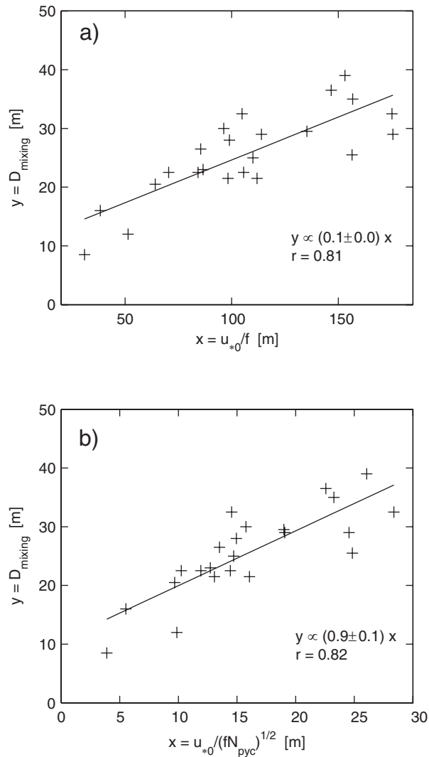
Figure 10. Regression of mixing layer depth, D_{\text{mixing}} , against a) outer neutral planetary length scale, u_{*0}/f , and b) stratified planetary length scale, u_{*0}/(fN_{\text{pyc}})^{1/2} . The slope ( \pm standard error) of the linear least-squares fit (with non-zero intercept) is indicated together with the correlation coefficient, r . When intercept is set to zero slopes are 0.23 ( r=0.65 ) and 1.5 ( r = 0.62 ), respectively, for a) and b).
