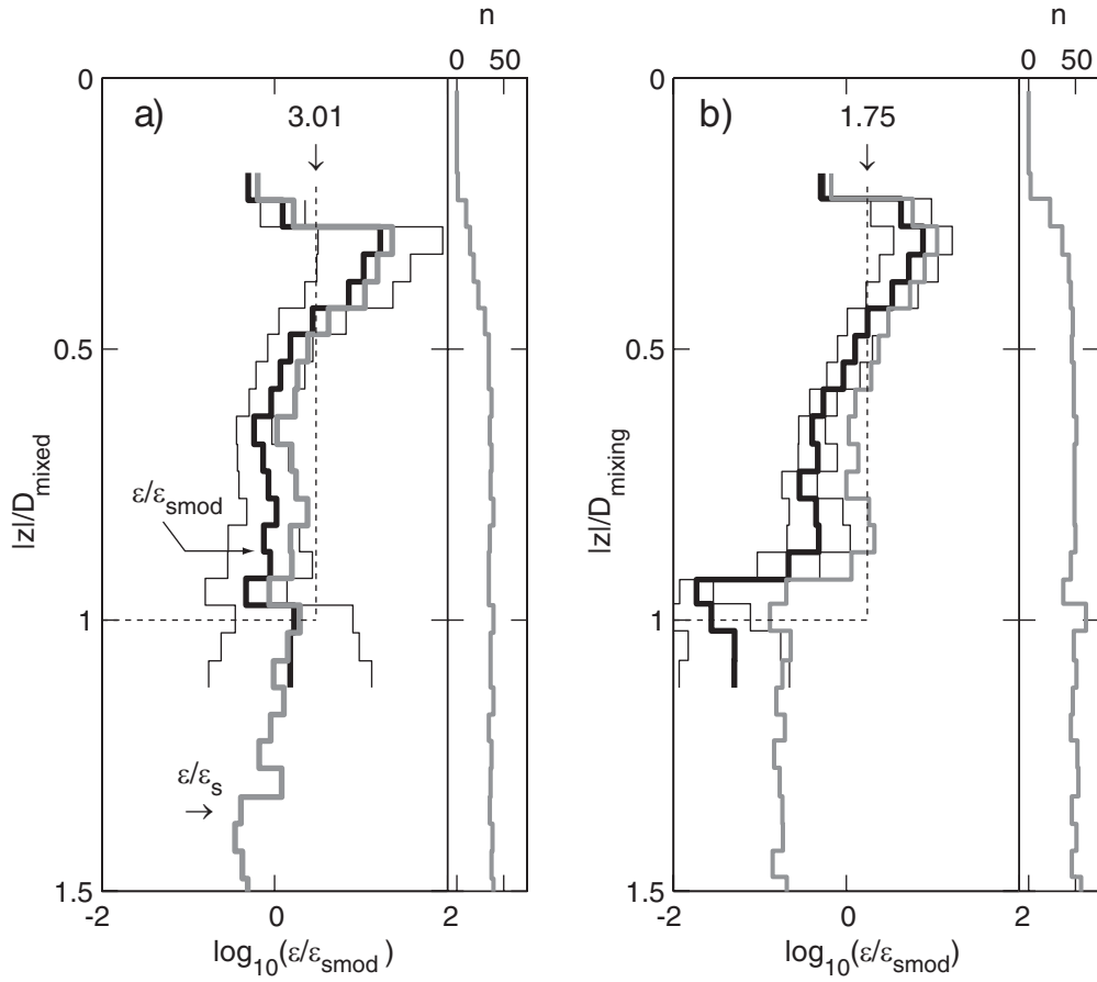
Figure 8. Profiles of dissipation rate \varepsilon normalized by the modified law-of-the wall \varepsilon_{\text{smod}} = u_{*0}^3/\lambda with \lambda from Eq. 5 (black). The distance from ice |z| is scaled by the mixed layer depth, D_{\text{mixed}} , in a) and by the mixing layer depth, D_{\text{mixing}} in b). The MLE values (black) and 95% confidence intervals are shown for |z|/D_{\text{mixing}} = 0.05 bins. There are typically \sim 50 data points, n , averaged in each normalized depth bin of the lower half of the mixed and mixing layers (narrow adjacent panels). The average of the standard LOW scaling (over both cases of ice relative speed in Figure 5) is shown for reference (gray).
